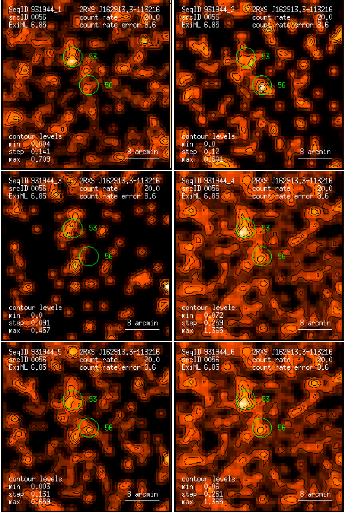
Figure 56: RASS 931944: detection 0056: band rate images, Gaussian filter: (1) PSPC channels 11 – 41, (2) 52 – 90, (3) 91 – 201, (4) 11 – 235, (5) 52 – 201, (6) 11 – 201. Broad band rates in counts/ks. Band rate contour levels in counts/ks/arcmin 2 .
