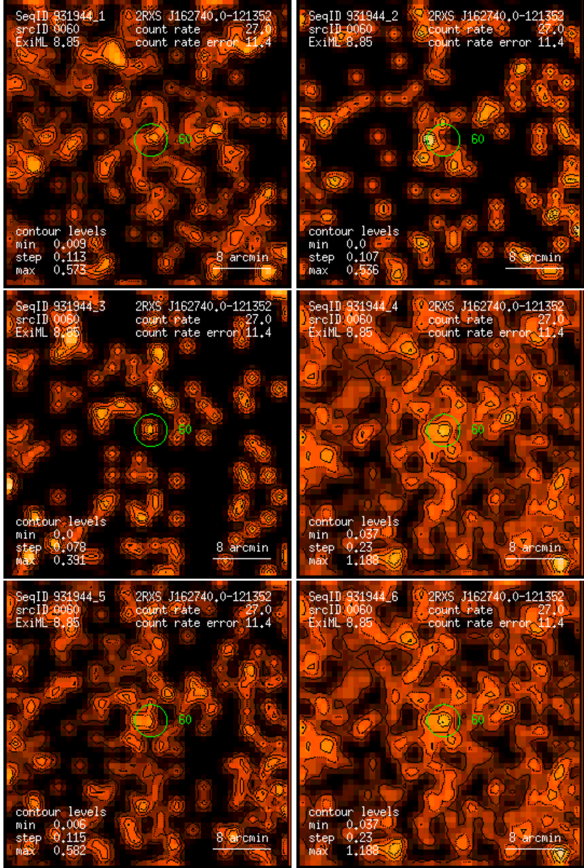
Figure 60: RASS 931944: detection 0060: band rate images, Gaussian filter: (1) PSPC channels 11 – 41, (2) 52 – 90, (3) 91 – 201, (4) 11 – 235, (5) 52 – 201, (6) 11 – 201. Broad band rates in counts/ks. Band rate contour levels in counts/ks/arcmin 2 .
