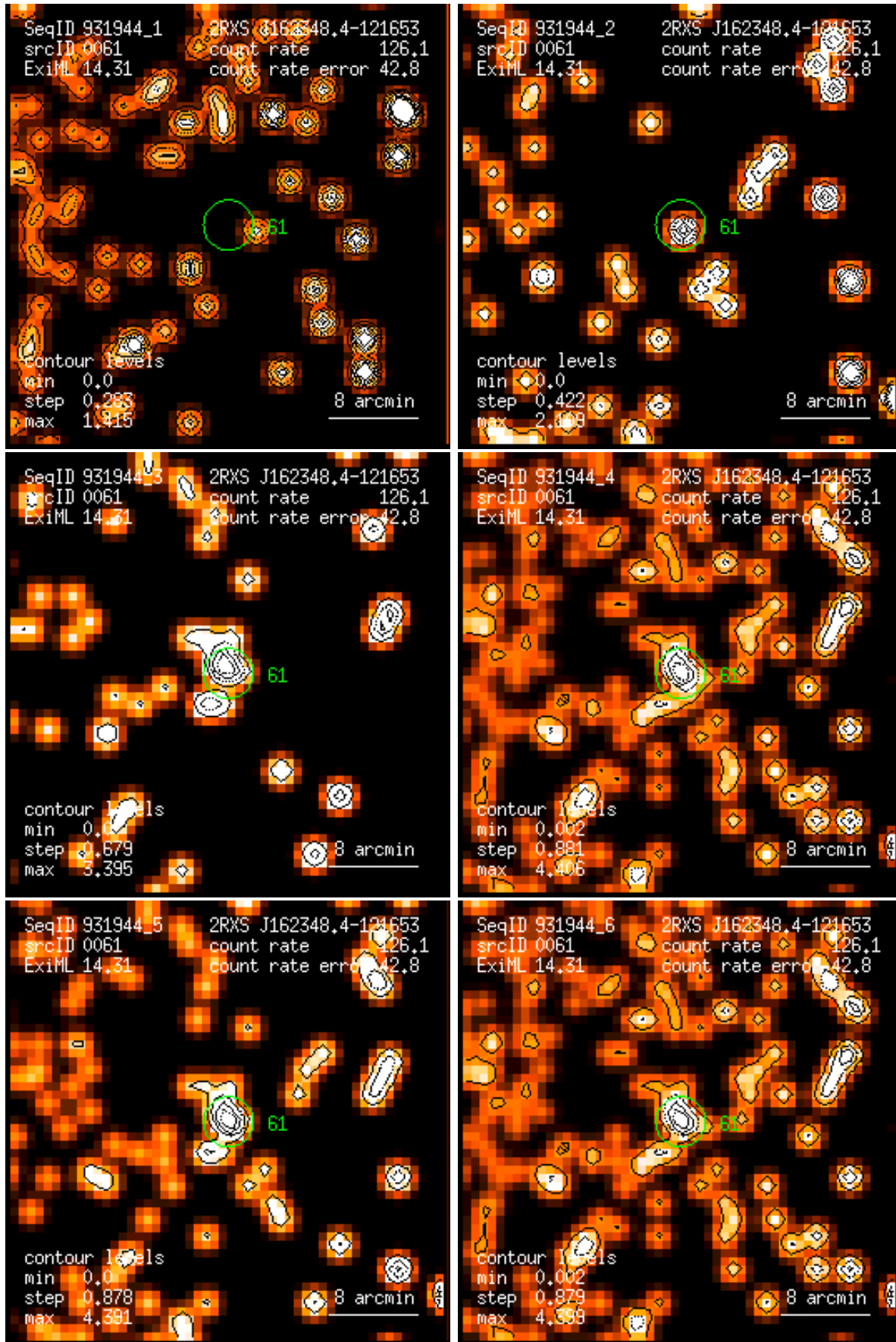
Figure 61: RASS 931944: detection 0061: band rate images, Gaussian filter: (1) PSPC channels 11 – 41, (2) 52 – 90, (3) 91 – 201, (4) 11 – 235, (5) 52 – 201, (6) 11 – 201. Broad band rates in counts/ks. Band rate contour levels in counts/ks/arcmin 2 .
