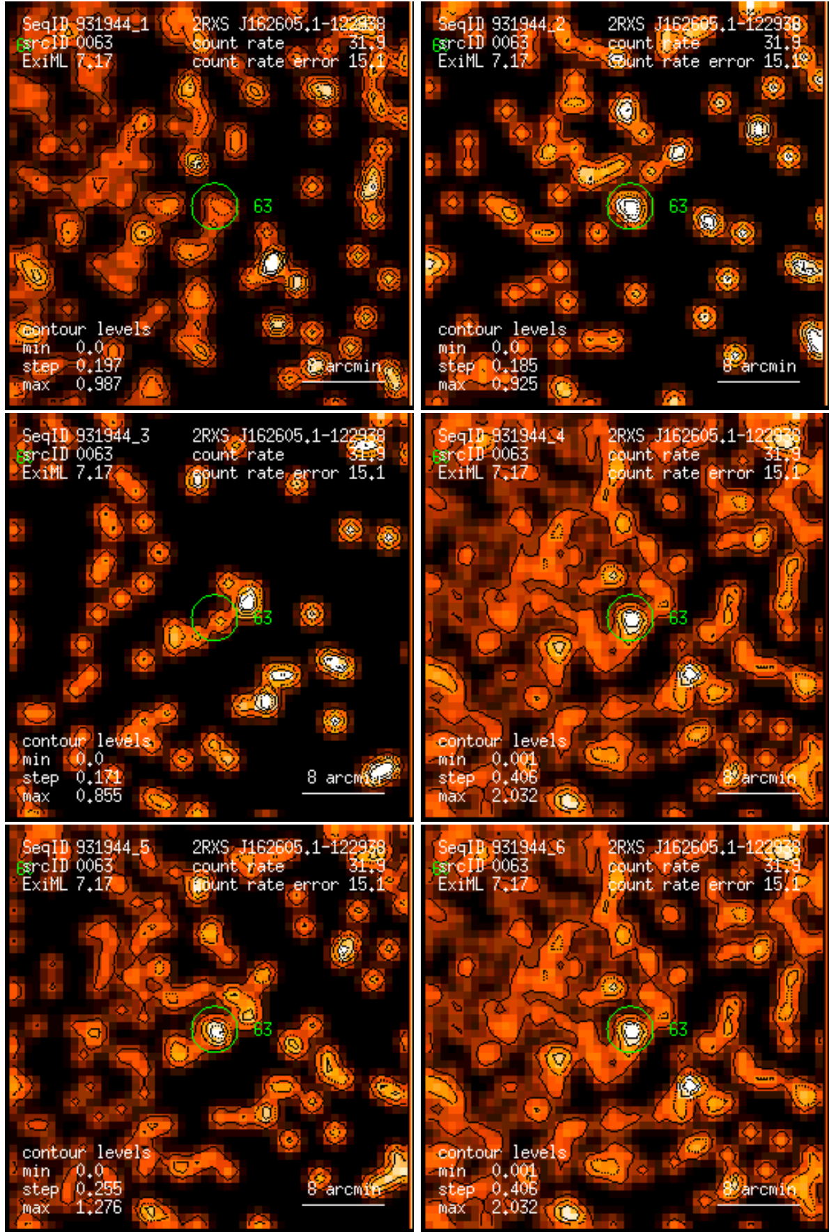
Figure 63: RASS 931944: detection 0063: band rate images, Gaussian filter: (1) PSPC channels 11 – 41, (2) 52 – 90, (3) 91 – 201, (4) 11 – 235, (5) 52 – 201, (6) 11 – 201. Broad band rates in counts/ks. Band rate contour levels in counts/ks/arcmin 2 .
