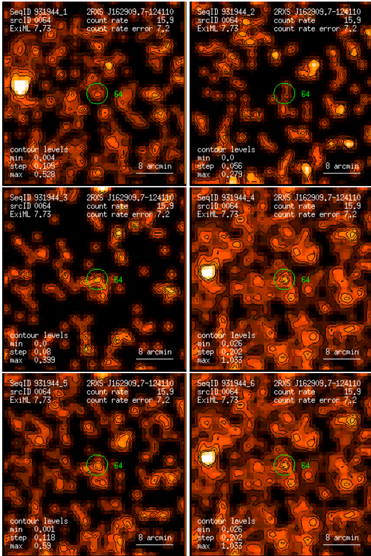
Figure 64: RASS 931944: detection 0064: band rate images, Gaussian filter: (1) PSPC channels 11 – 41, (2) 52 – 90, (3) 91 – 201, (4) 11 – 235, (5) 52 – 201, (6) 11 – 201. Broad band rates in counts/ks. Band rate contour levels in counts/ks/arcmin 2 .
