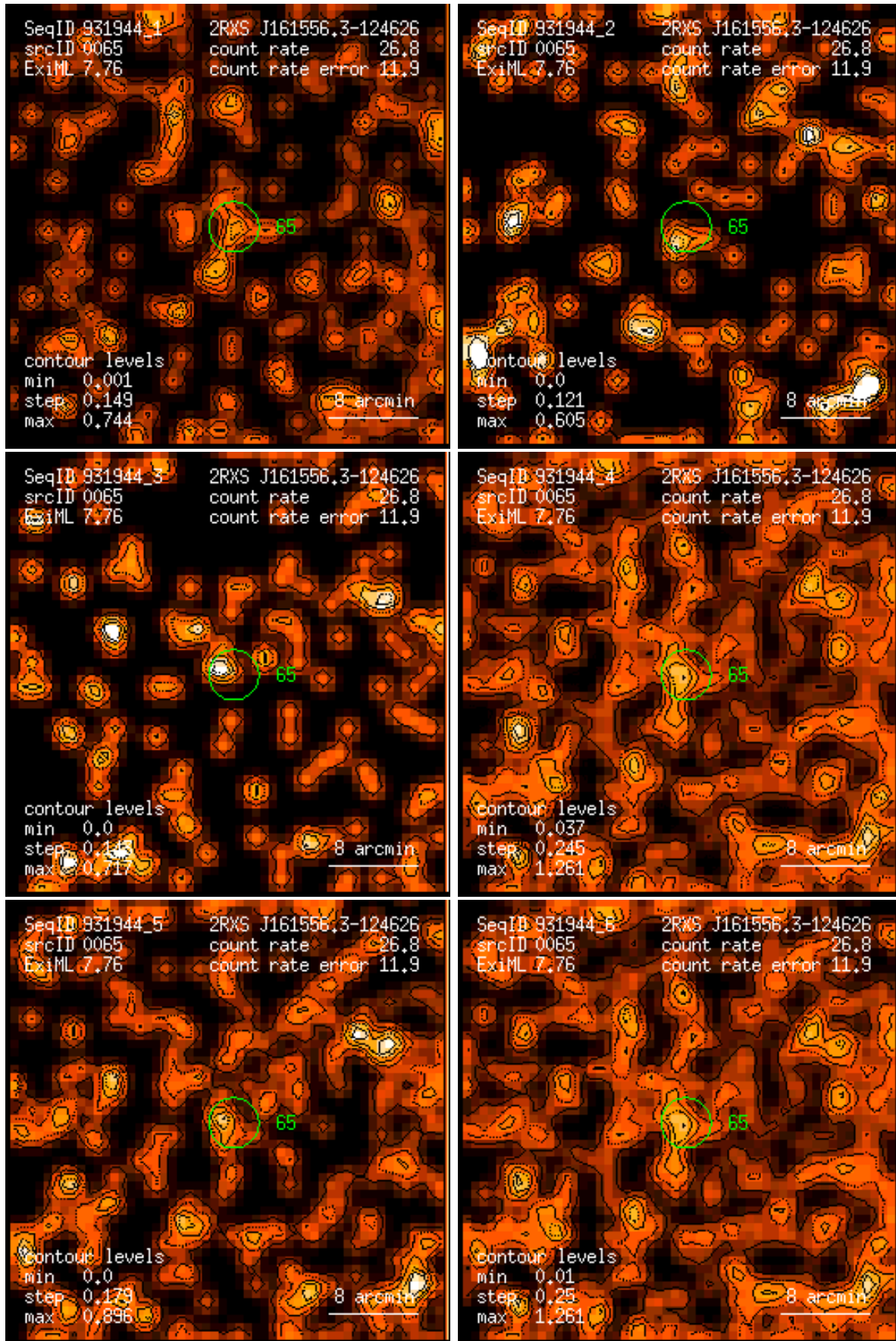
Figure 65: RASS 931944: detection 0065: band rate images, Gaussian filter: (1) PSPC channels 11 – 41, (2) 52 – 90, (3) 91 – 201, (4) 11 – 235, (5) 52 – 201, (6) 11 – 201. Broad band rates in counts/ks. Band rate contour levels in counts/ks/arcmin 2 .
