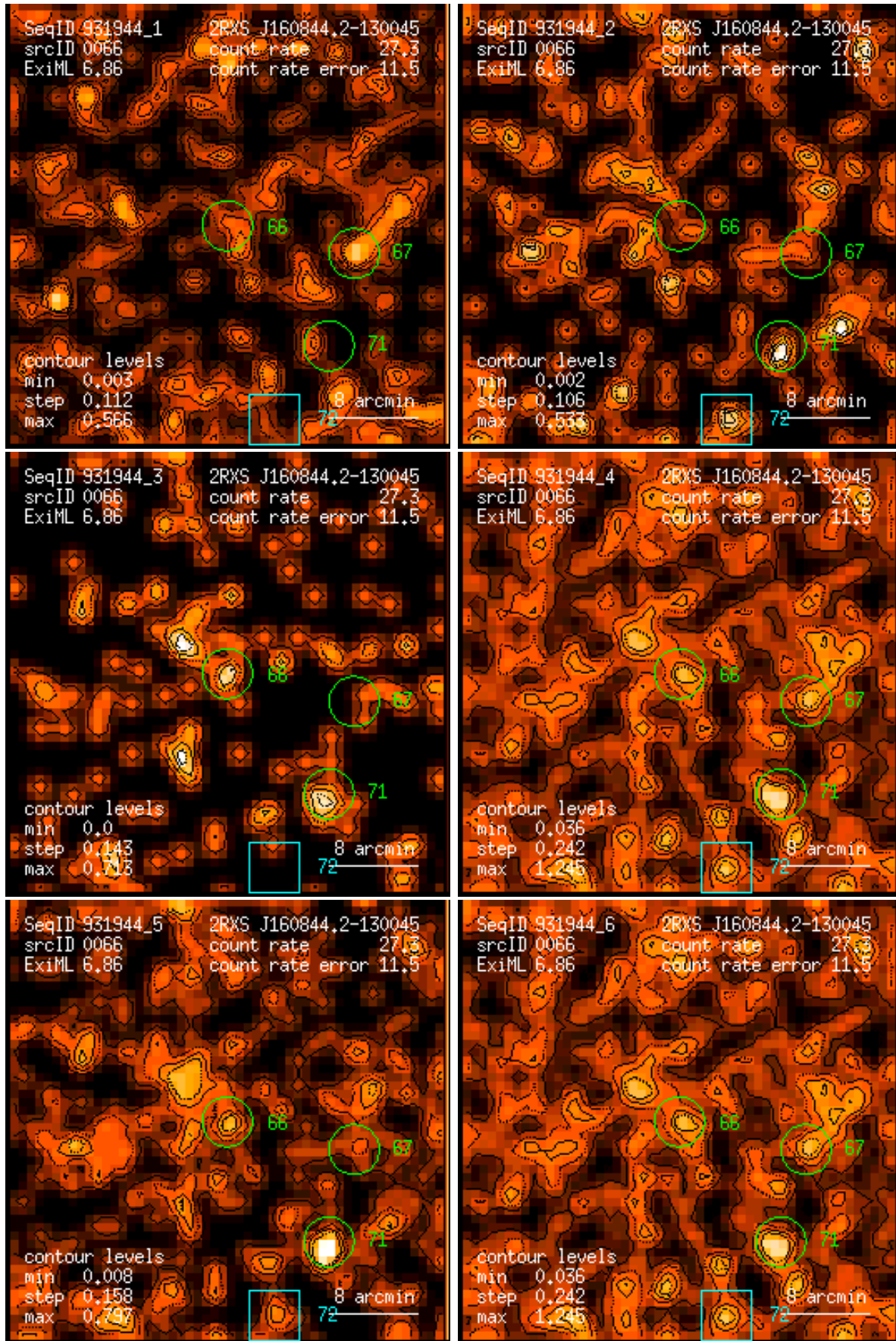
Figure 66: RASS 931944: detection 0066: band rate images, Gaussian filter: (1) PSPC channels 11 – 41, (2) 52 – 90, (3) 91 – 201, (4) 11 – 235, (5) 52 – 201, (6) 11 – 201. Broad band rates in counts/ks. Band rate contour levels in counts/ks/arcmin 2 .
