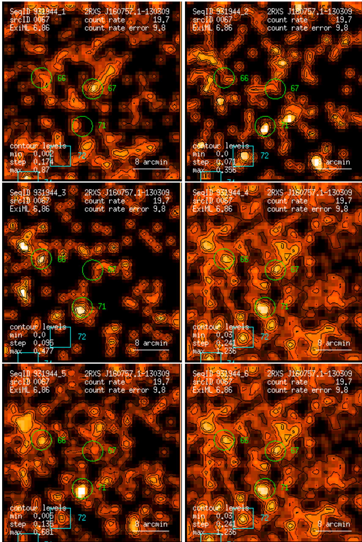
Figure 67: RASS 931944: detection 0067: band rate images, Gaussian filter: (1) PSPC channels 11 – 41, (2) 52 – 90, (3) 91 – 201, (4) 11 – 235, (5) 52 – 201, (6) 11 – 201. Broad band rates in counts/ks. Band rate contour levels in counts/ks/arcmin 2 .
