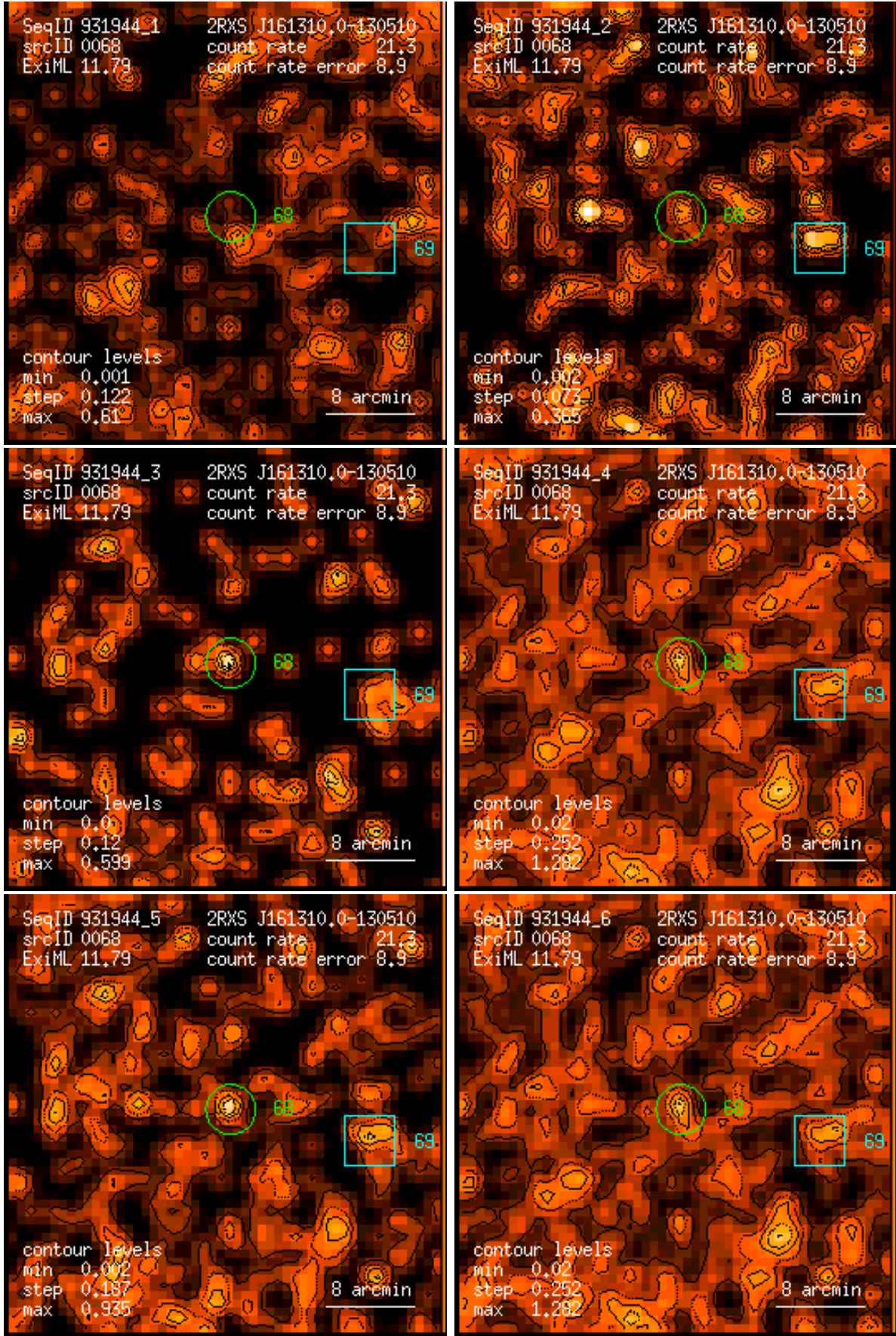
Figure 68: RASS 931944: detection 0068: band rate images, Gaussian filter: (1) PSPC channels 11 – 41, (2) 52 – 90, (3) 91 – 201, (4) 11 – 235, (5) 52 – 201, (6) 11 – 201. Broad band rates in counts/ks. Band rate contour levels in counts/ks/arcmin 2 .
