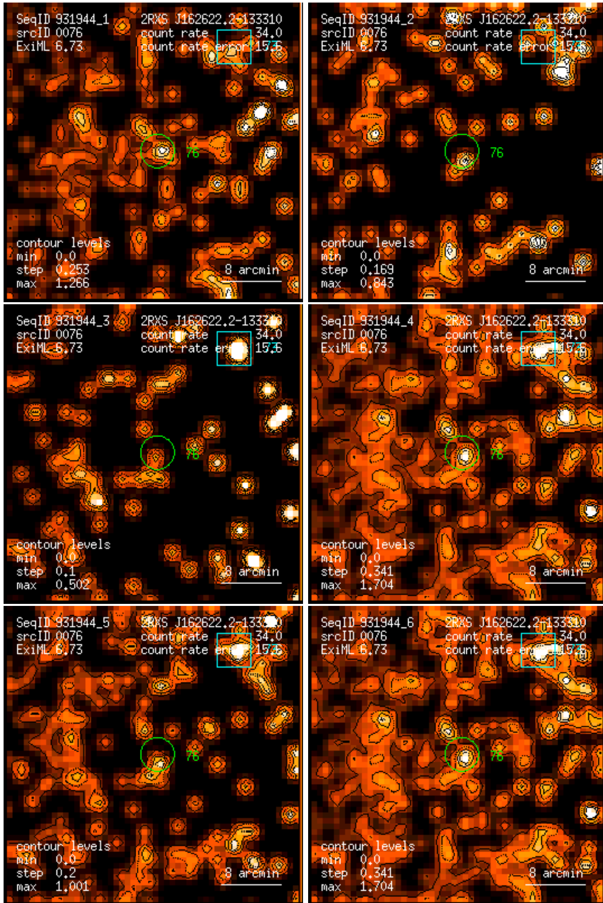
Figure 76: RASS 931944: detection 0076: band rate images, Gaussian filter: (1) PSPC channels 11 – 41, (2) 52 – 90, (3) 91 – 201, (4) 11 – 235, (5) 52 – 201, (6) 11 – 201. Broad band rates in counts/ks. Band rate contour levels in counts/ks/arcmin 2 .
