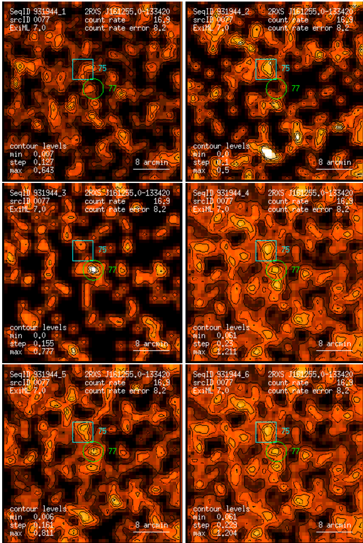
Figure 77: RASS 931944: detection 0077: band rate images, Gaussian filter: (1) PSPC channels 11 – 41, (2) 52 – 90, (3) 91 – 201, (4) 11 – 235, (5) 52 – 201, (6) 11 – 201. Broad band rates in counts/ks. Band rate contour levels in counts/ks/arcmin 2 .
