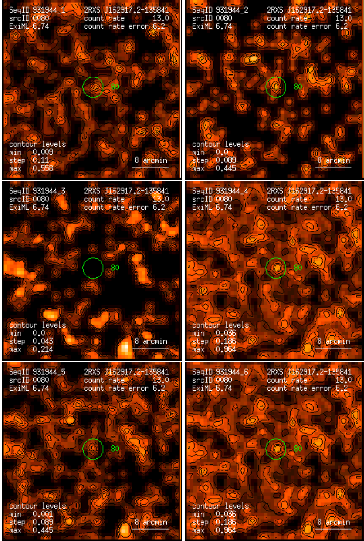
Figure 80: RASS 931944: detection 0080: band rate images, Gaussian filter: (1) PSPC channels 11 – 41, (2) 52 – 90, (3) 91 – 201, (4) 11 – 235, (5) 52 – 201, (6) 11 – 201. Broad band rates in counts/ks. Band rate contour levels in counts/ks/arcmin 2 .
