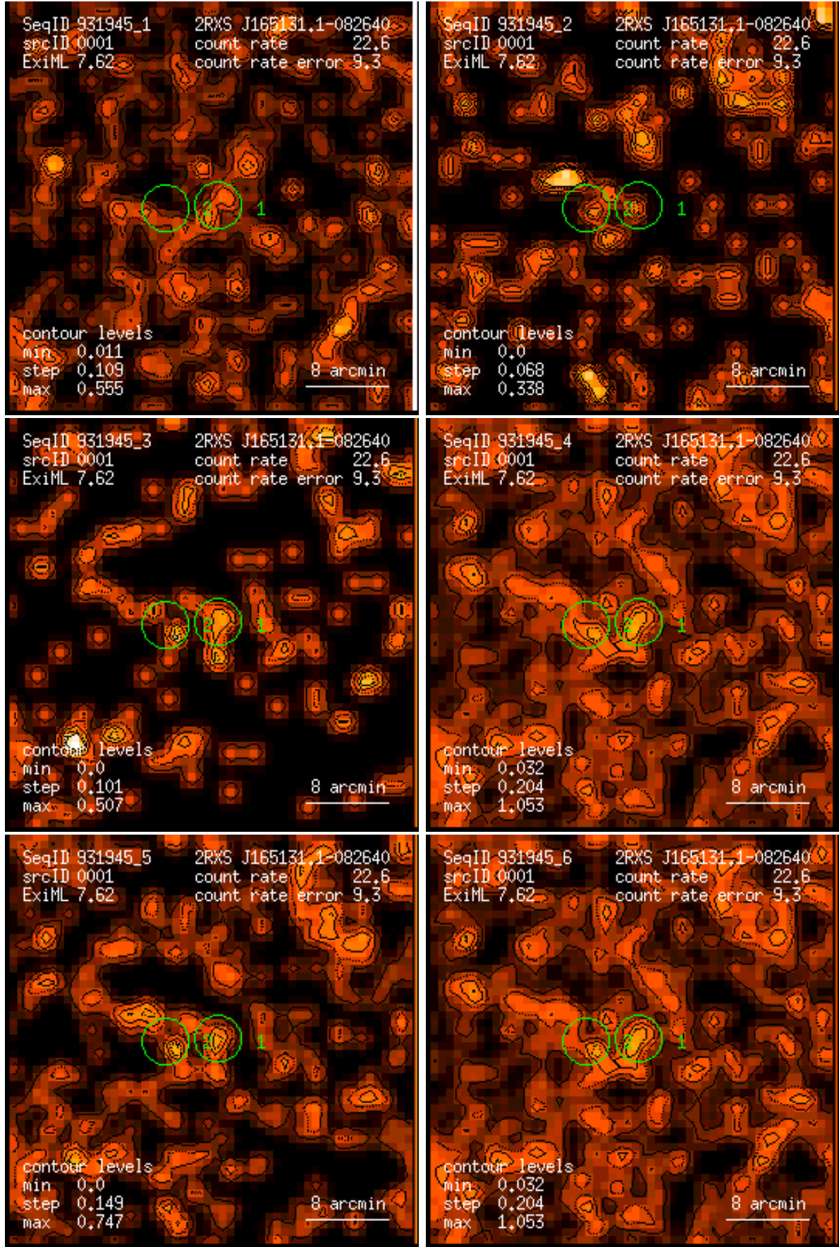
Figure 1: RASS 931945: detection 0001: band rate images, Gaussian filter: (1) PSPC channels 11 – 41, (2) 52 – 90, (3) 91 – 201, (4) 11 – 235, (5) 52 – 201, (6) 11 – 201. Broad band rates in counts/ks. Band rate contour levels in counts/ks/arcmin 2 .
