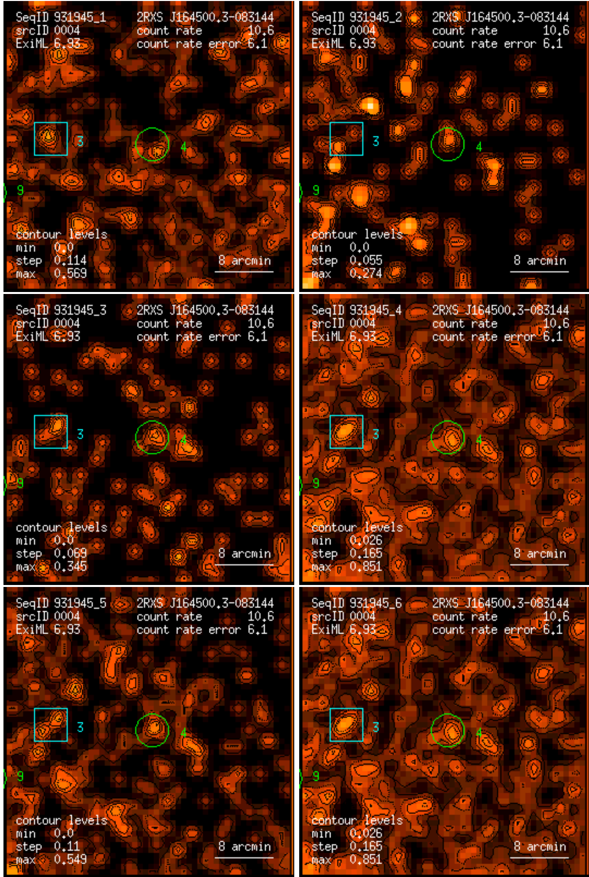
Figure 4: RASS 931945: detection 0004: band rate images, Gaussian filter: (1) PSPC channels 11 – 41, (2) 52 – 90, (3) 91 – 201, (4) 11 – 235, (5) 52 – 201, (6) 11 – 201. Broad band rates in counts/ks. Band rate contour levels in counts/ks/arcmin 2 .
