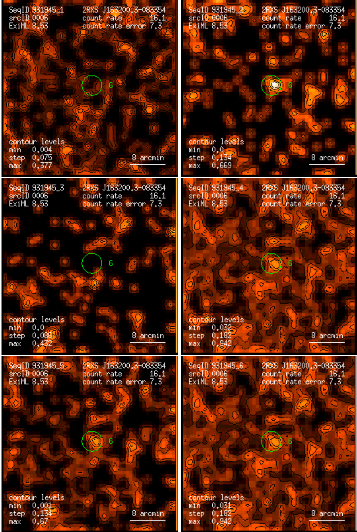
Figure 6: RASS 931945: detection 0006: band rate images, Gaussian filter: (1) PSPC channels 11 – 41, (2) 52 – 90, (3) 91 – 201, (4) 11 – 235, (5) 52 – 201, (6) 11 – 201. Broad band rates in counts/ks. Band rate contour levels in counts/ks/arcmin 2 .
