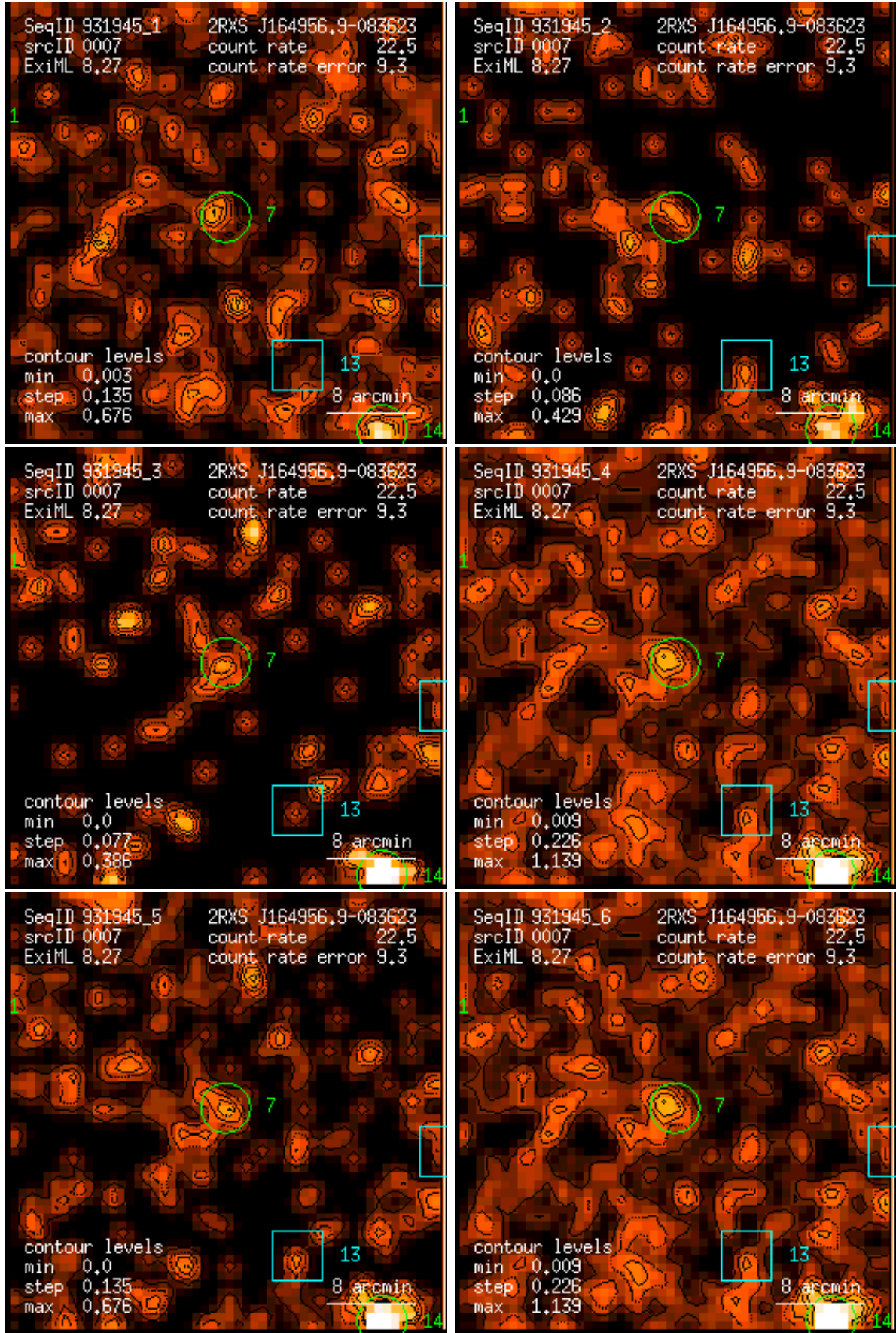
Figure 7: RASS 931945: detection 0007: band rate images, Gaussian filter: (1) PSPC channels 11 – 41, (2) 52 – 90, (3) 91 – 201, (4) 11 – 235, (5) 52 – 201, (6) 11 – 201. Broad band rates in counts/ks. Band rate contour levels in counts/ks/arcmin 2 .
