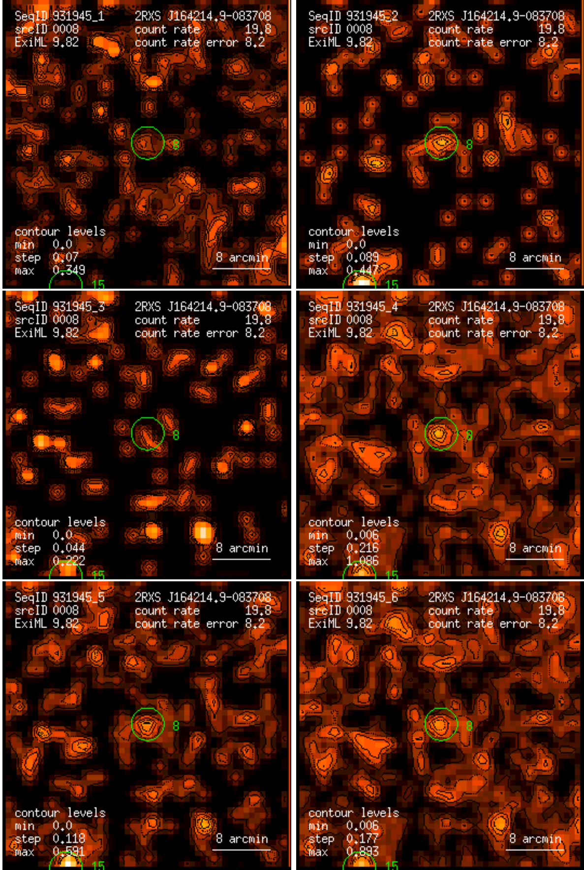
Figure 8: RASS 931945: detection 0008: band rate images, Gaussian filter: (1) PSPC channels 11 – 41, (2) 52 – 90, (3) 91 – 201, (4) 11 – 235, (5) 52 – 201, (6) 11 – 201. Broad band rates in counts/ks. Band rate contour levels in counts/ks/arcmin 2 .
