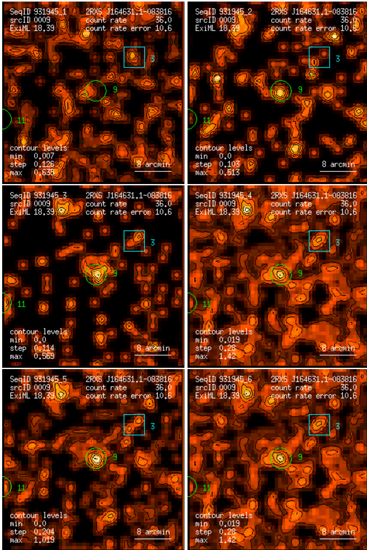
Figure 9: RASS 931945: detection 0009: band rate images, Gaussian filter: (1) PSPC channels 11 – 41, (2) 52 – 90, (3) 91 – 201, (4) 11 – 235, (5) 52 – 201, (6) 11 – 201. Broad band rates in counts/ks. Band rate contour levels in counts/ks/arcmin 2 .
