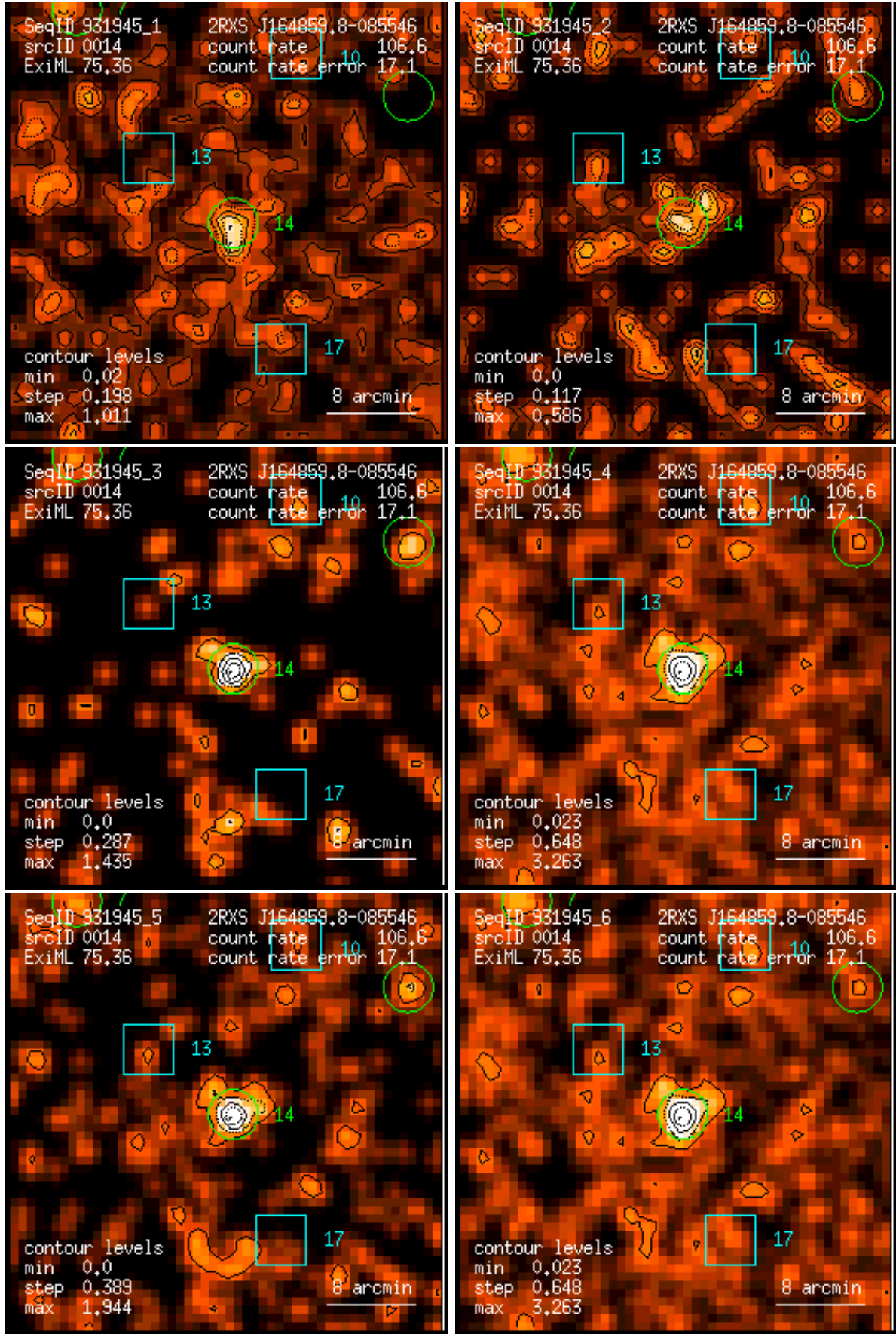
Figure 14: RASS 931945: detection 0014: band rate images, Gaussian filter: (1) PSPC channels 11 – 41, (2) 52 – 90, (3) 91 – 201, (4) 11 – 235, (5) 52 – 201, (6) 11 – 201. Broad band rates in counts/ks. Band rate contour levels in counts/ks/arcmin 2 .
