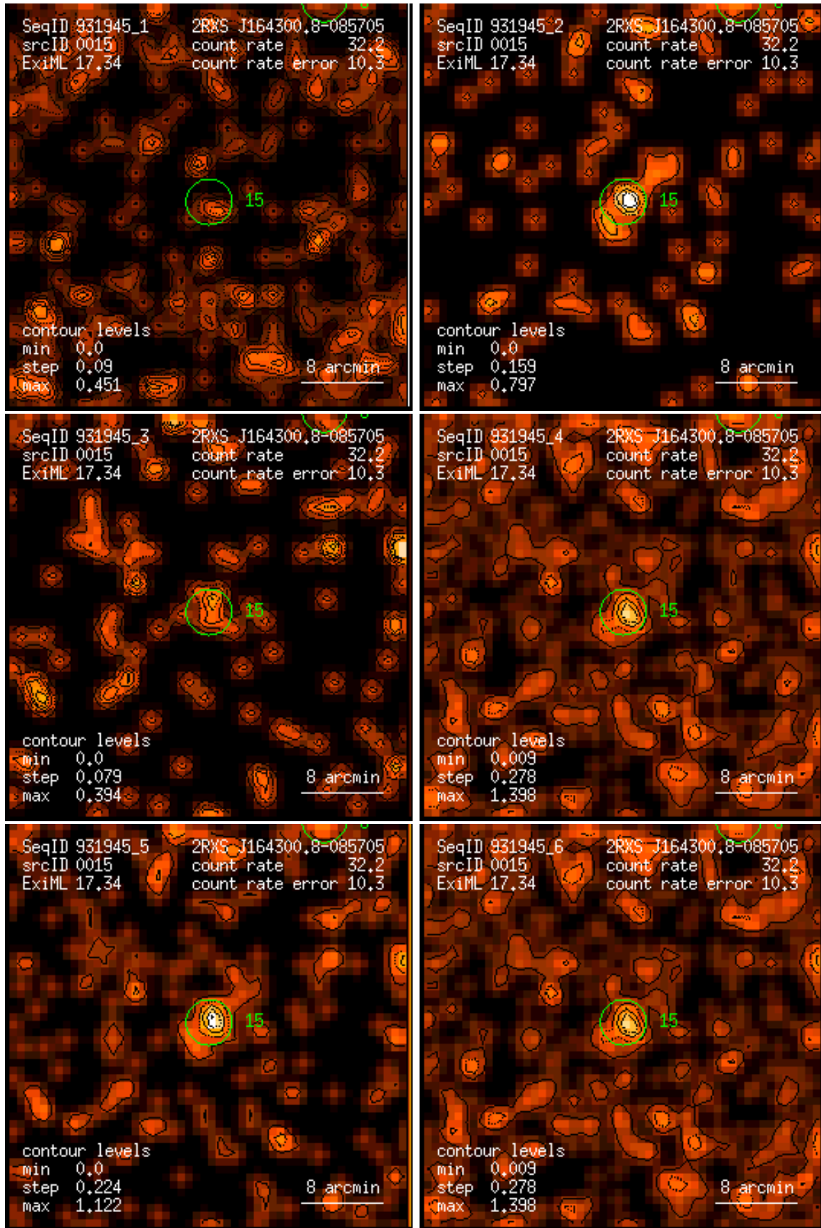
Figure 15: RASS 931945: detection 0015: band rate images, Gaussian filter: (1) PSPC channels 11 – 41, (2) 52 – 90, (3) 91 – 201, (4) 11 – 235, (5) 52 – 201, (6) 11 – 201. Broad band rates in counts/ks. Band rate contour levels in counts/ks/arcmin 2 .
