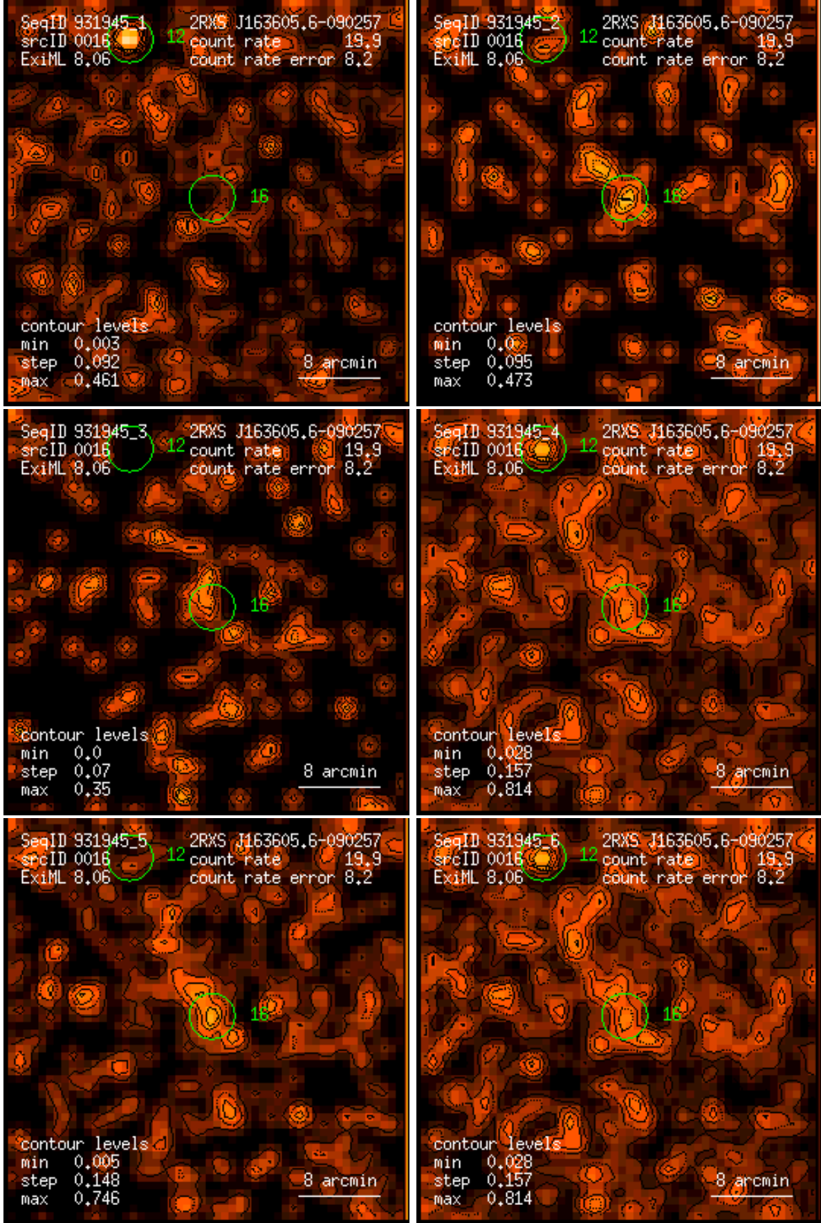
Figure 16: RASS 931945: detection 0016: band rate images, Gaussian filter: (1) PSPC channels 11 – 41, (2) 52 – 90, (3) 91 – 201, (4) 11 – 235, (5) 52 – 201, (6) 11 – 201. Broad band rates in counts/ks. Band rate contour levels in counts/ks/arcmin 2 .
