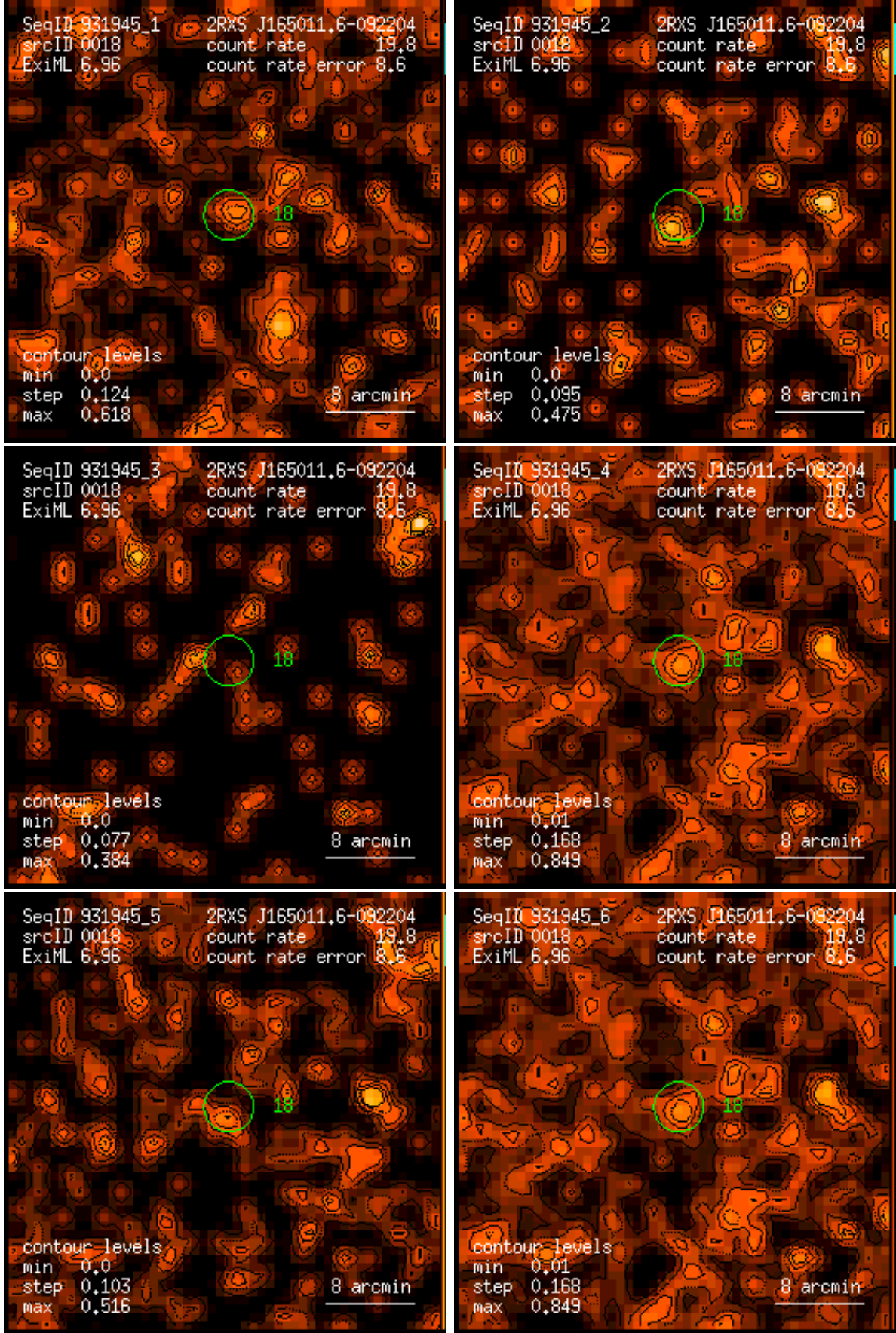
Figure 18: RASS 931945: detection 0018: band rate images, Gaussian filter: (1) PSPC channels 11 – 41, (2) 52 – 90, (3) 91 – 201, (4) 11 – 235, (5) 52 – 201, (6) 11 – 201. Broad band rates in counts/ks. Band rate contour levels in counts/ks/arcmin 2 .
