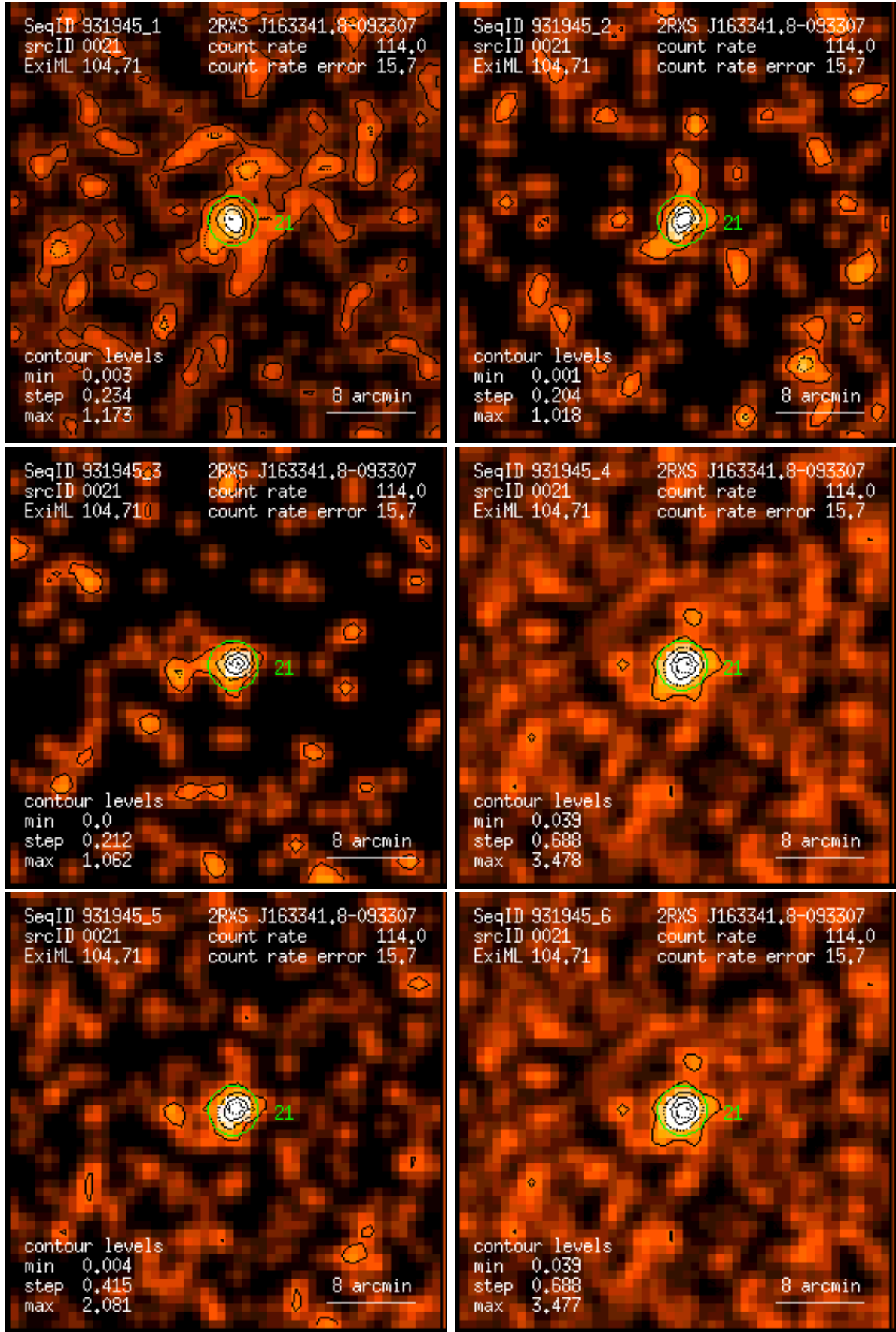
Figure 21: RASS 931945: detection 0021: band rate images, Gaussian filter: (1) PSPC channels 11 – 41, (2) 52 – 90, (3) 91 – 201, (4) 11 – 235, (5) 52 – 201, (6) 11 – 201. Broad band rates in counts/ks. Band rate contour levels in counts/ks/arcmin 2 .
