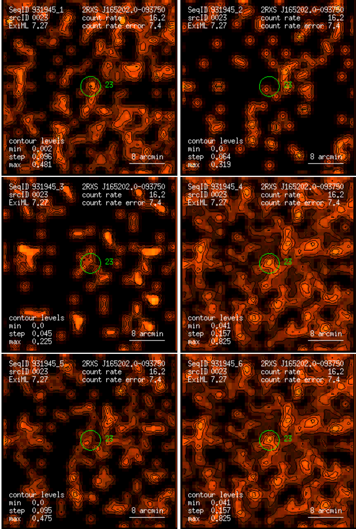
Figure 23: RASS 931945: detection 0023: band rate images, Gaussian filter: (1) PSPC channels 11 – 41, (2) 52 – 90, (3) 91 – 201, (4) 11 – 235, (5) 52 – 201, (6) 11 – 201. Broad band rates in counts/ks. Band rate contour levels in counts/ks/arcmin 2 .
