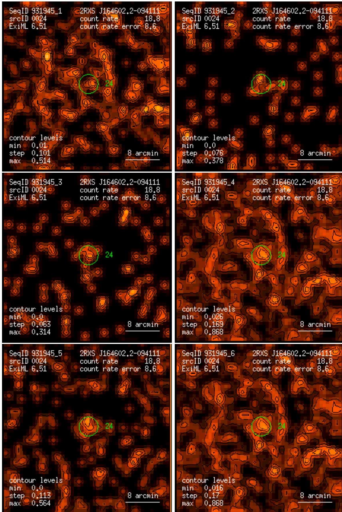
Figure 24: RASS 931945: detection 0024: band rate images, Gaussian filter: (1) PSPC channels 11 – 41, (2) 52 – 90, (3) 91 – 201, (4) 11 – 235, (5) 52 – 201, (6) 11 – 201. Broad band rates in counts/ks. Band rate contour levels in counts/ks/arcmin 2 .
