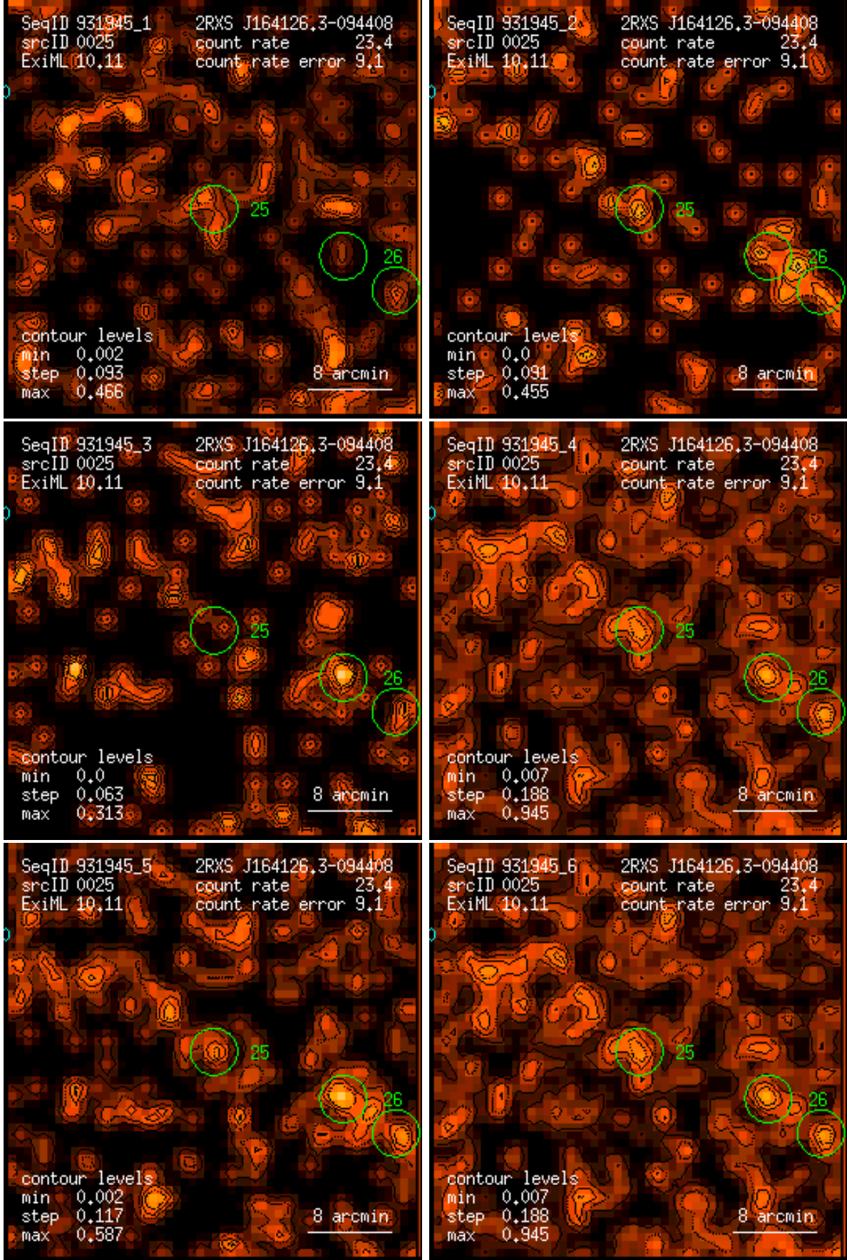
Figure 25: RASS 931945: detection 0025: band rate images, Gaussian filter: (1) PSPC channels 11 – 41, (2) 52 – 90, (3) 91 – 201, (4) 11 – 235, (5) 52 – 201, (6) 11 – 201. Broad band rates in counts/ks. Band rate contour levels in counts/ks/arcmin 2 .
