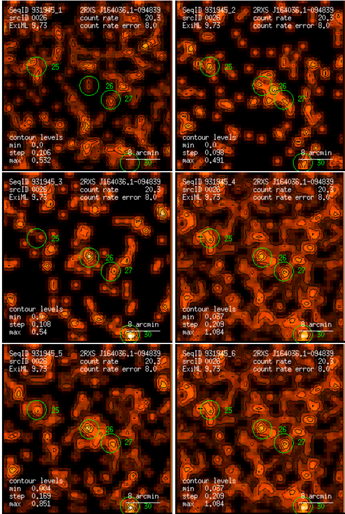
Figure 26: RASS 931945: detection 0026: band rate images, Gaussian filter: (1) PSPC channels 11 – 41, (2) 52 – 90, (3) 91 – 201, (4) 11 – 235, (5) 52 – 201, (6) 11 – 201. Broad band rates in counts/ks. Band rate contour levels in counts/ks/arcmin 2 .
