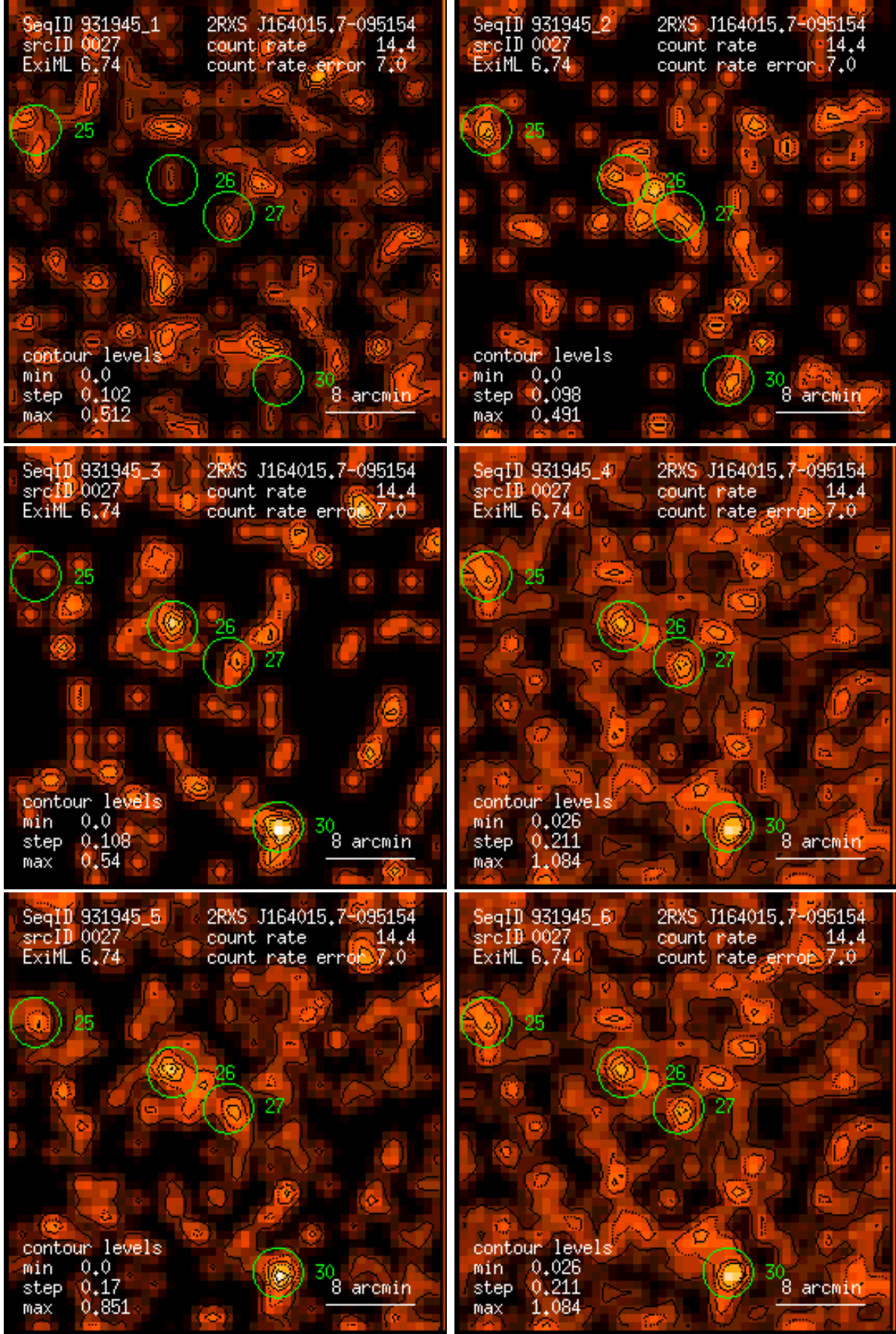
Figure 27: RASS 931945: detection 0027: band rate images, Gaussian filter: (1) PSPC channels 11 – 41, (2) 52 – 90, (3) 91 – 201, (4) 11 – 235, (5) 52 – 201, (6) 11 – 201. Broad band rates in counts/ks. Band rate contour levels in counts/ks/arcmin 2 .
