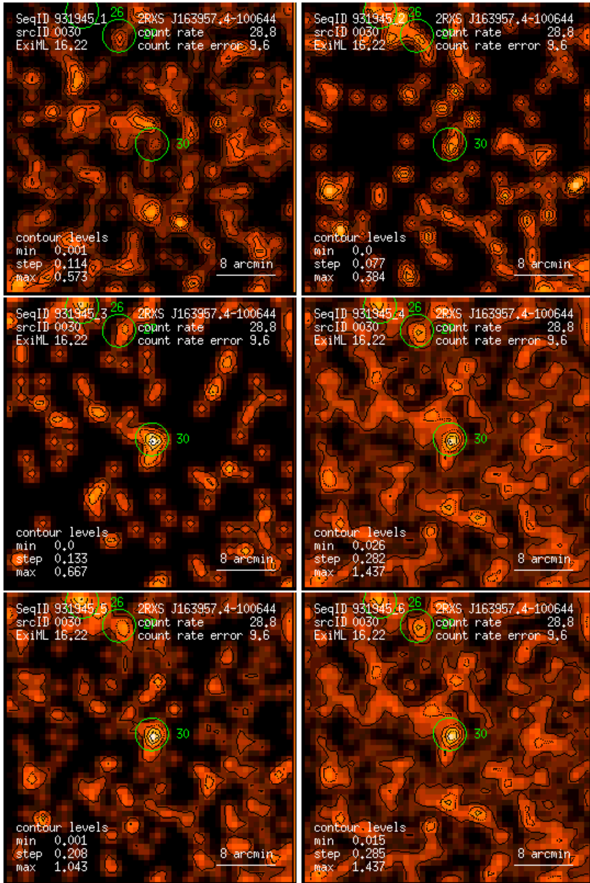
Figure 30: RASS 931945: detection 0030: band rate images, Gaussian filter: (1) PSPC channels 11 – 41, (2) 52 – 90, (3) 91 – 201, (4) 11 – 235, (5) 52 – 201, (6) 11 – 201. Broad band rates in counts/ks. Band rate contour levels in counts/ks/arcmin 2 .
