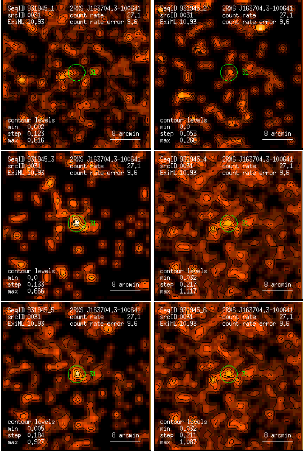
Figure 31: RASS 931945: detection 0031: band rate images, Gaussian filter: (1) PSPC channels 11 – 41, (2) 52 – 90, (3) 91 – 201, (4) 11 – 235, (5) 52 – 201, (6) 11 – 201. Broad band rates in counts/ks. Band rate contour levels in counts/ks/arcmin 2 .
