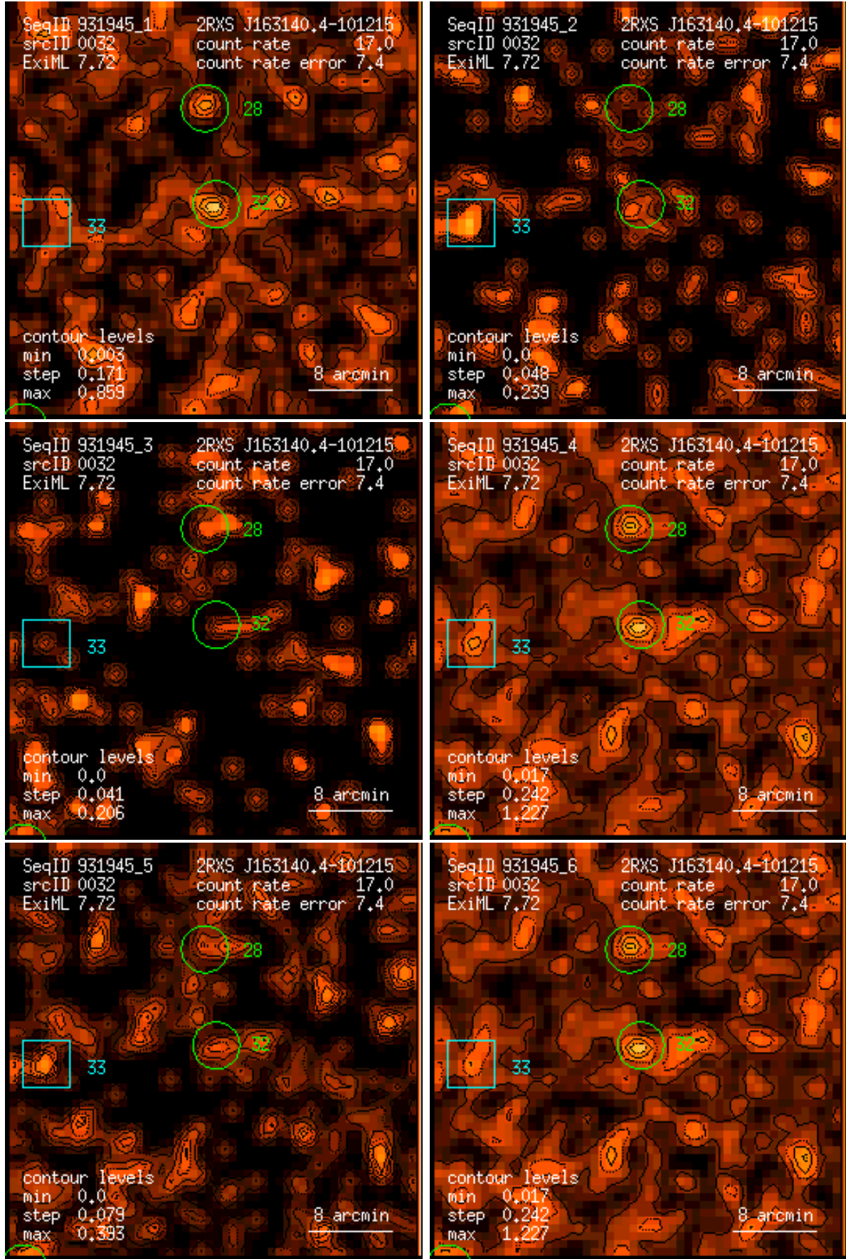
Figure 32: RASS 931945: detection 0032: band rate images, Gaussian filter: (1) PSPC channels 11 – 41, (2) 52 – 90, (3) 91 – 201, (4) 11 – 235, (5) 52 – 201, (6) 11 – 201. Broad band rates in counts/ks. Band rate contour levels in counts/ks/arcmin 2 .
