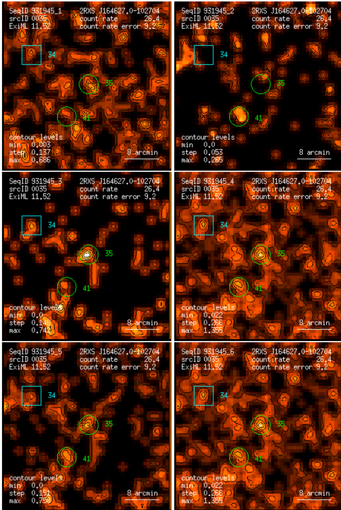
Figure 35: RASS 931945: detection 0035: band rate images, Gaussian filter: (1) PSPC channels 11 – 41, (2) 52 – 90, (3) 91 – 201, (4) 11 – 235, (5) 52 – 201, (6) 11 – 201. Broad band rates in counts/ks. Band rate contour levels in counts/ks/arcmin 2 .
