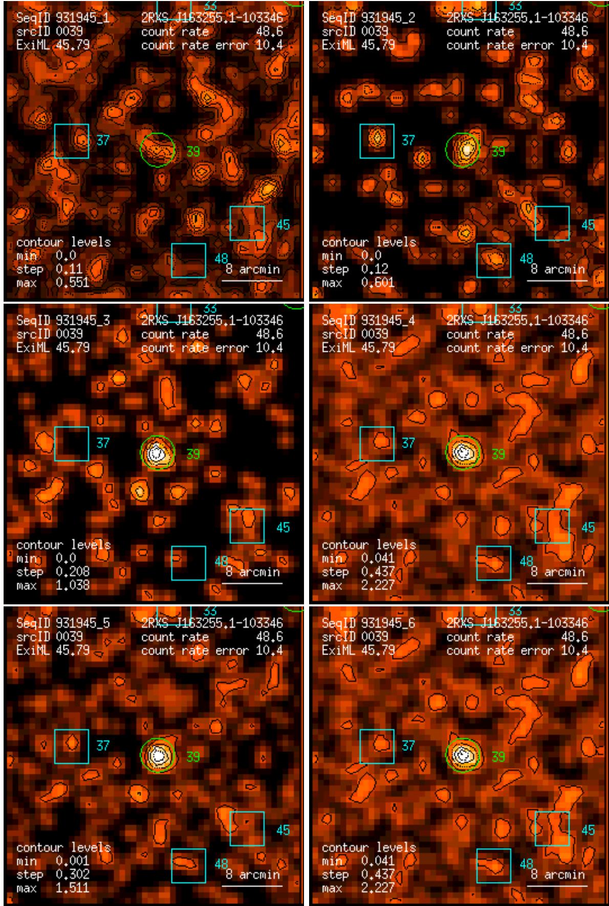
Figure 39: RASS 931945: detection 0039: band rate images, Gaussian filter: (1) PSPC channels 11 – 41, (2) 52 – 90, (3) 91 – 201, (4) 11 – 235, (5) 52 – 201, (6) 11 – 201. Broad band rates in counts/ks. Band rate contour levels in counts/ks/arcmin 2 .
