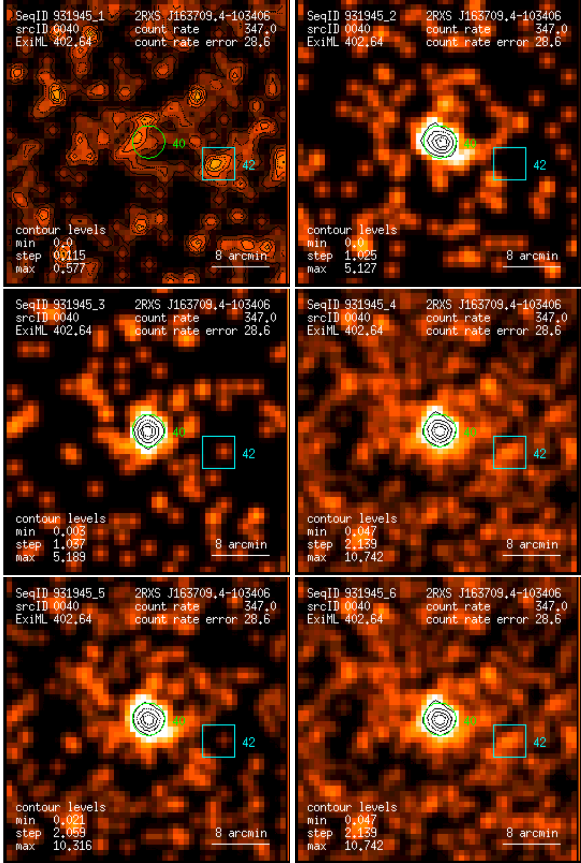
Figure 40: RASS 931945: detection 0040: band rate images, Gaussian filter: (1) PSPC channels 11 – 41, (2) 52 – 90, (3) 91 – 201, (4) 11 – 235, (5) 52 – 201, (6) 11 – 201. Broad band rates in counts/ks. Band rate contour levels in counts/ks/arcmin 2 .
