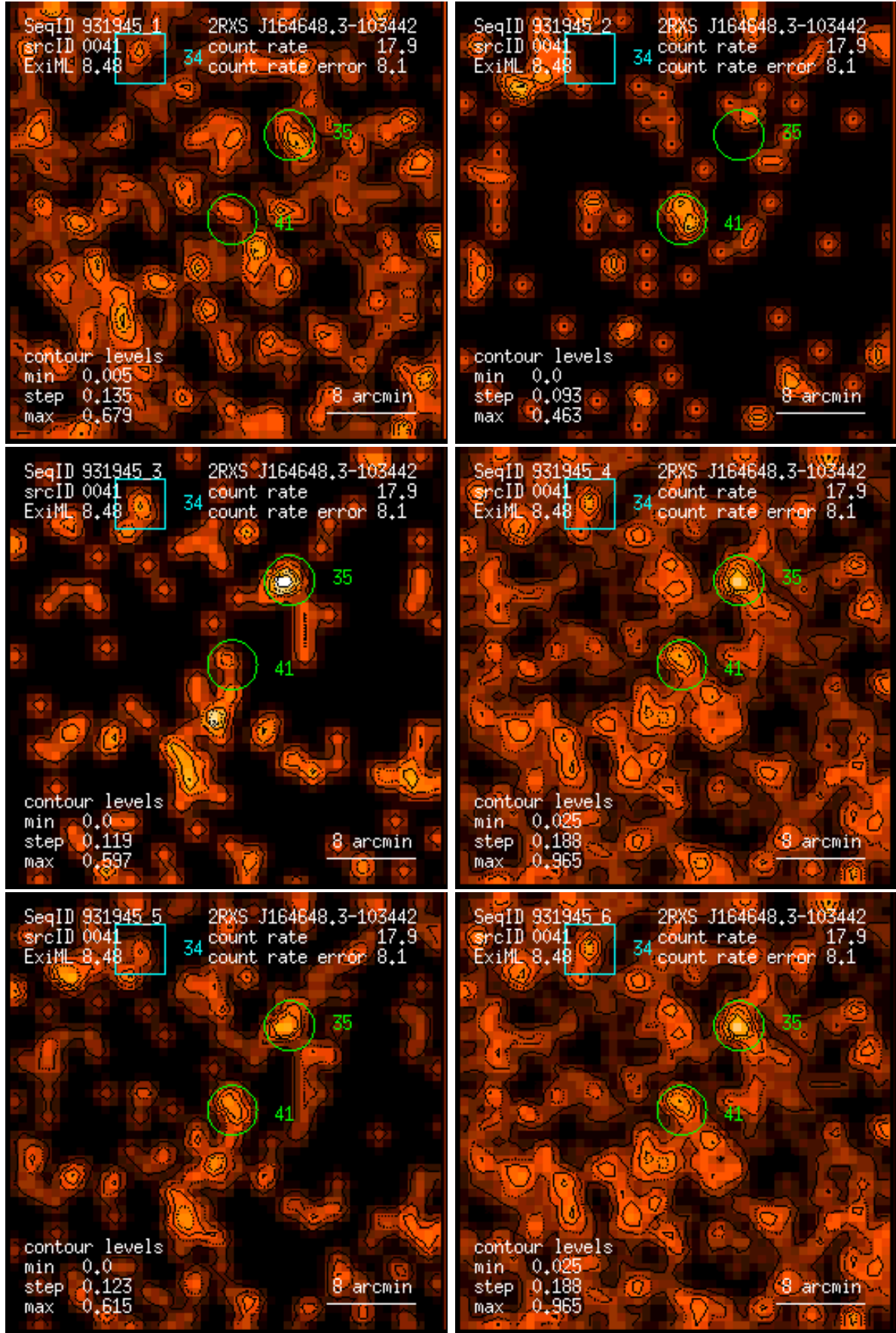
Figure 41: RASS 931945: detection 0041: band rate images, Gaussian filter: (1) PSPC channels 11 – 41, (2) 52 – 90, (3) 91 – 201, (4) 11 – 235, (5) 52 – 201, (6) 11 – 201. Broad band rates in counts/ks. Band rate contour levels in counts/ks/arcmin 2 .
