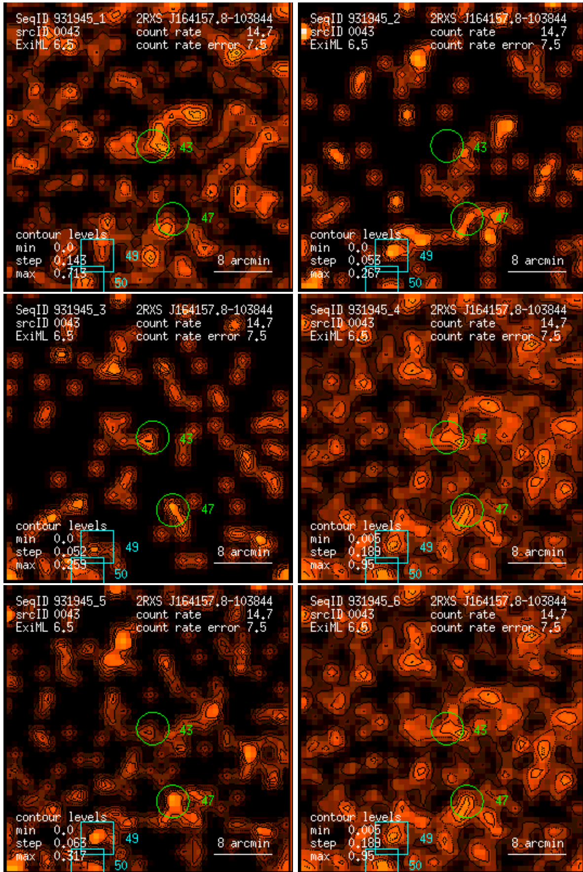
Figure 43: RASS 931945: detection 0043: band rate images, Gaussian filter: (1) PSPC channels 11 – 41, (2) 52 – 90, (3) 91 – 201, (4) 11 – 235, (5) 52 – 201, (6) 11 – 201. Broad band rates in counts/ks. Band rate contour levels in counts/ks/arcmin 2 .
