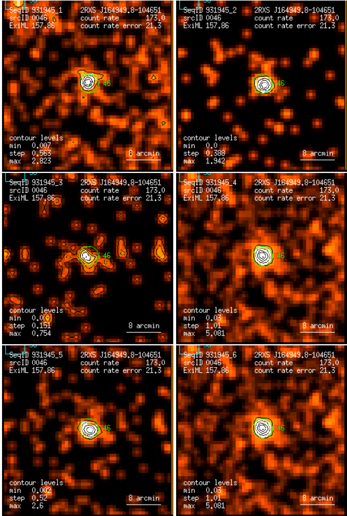
Figure 46: RASS 931945: detection 0046: band rate images, Gaussian filter: (1) PSPC channels 11 – 41, (2) 52 – 90, (3) 91 – 201, (4) 11 – 235, (5) 52 – 201, (6) 11 – 201. Broad band rates in counts/ks. Band rate contour levels in counts/ks/arcmin 2 .
