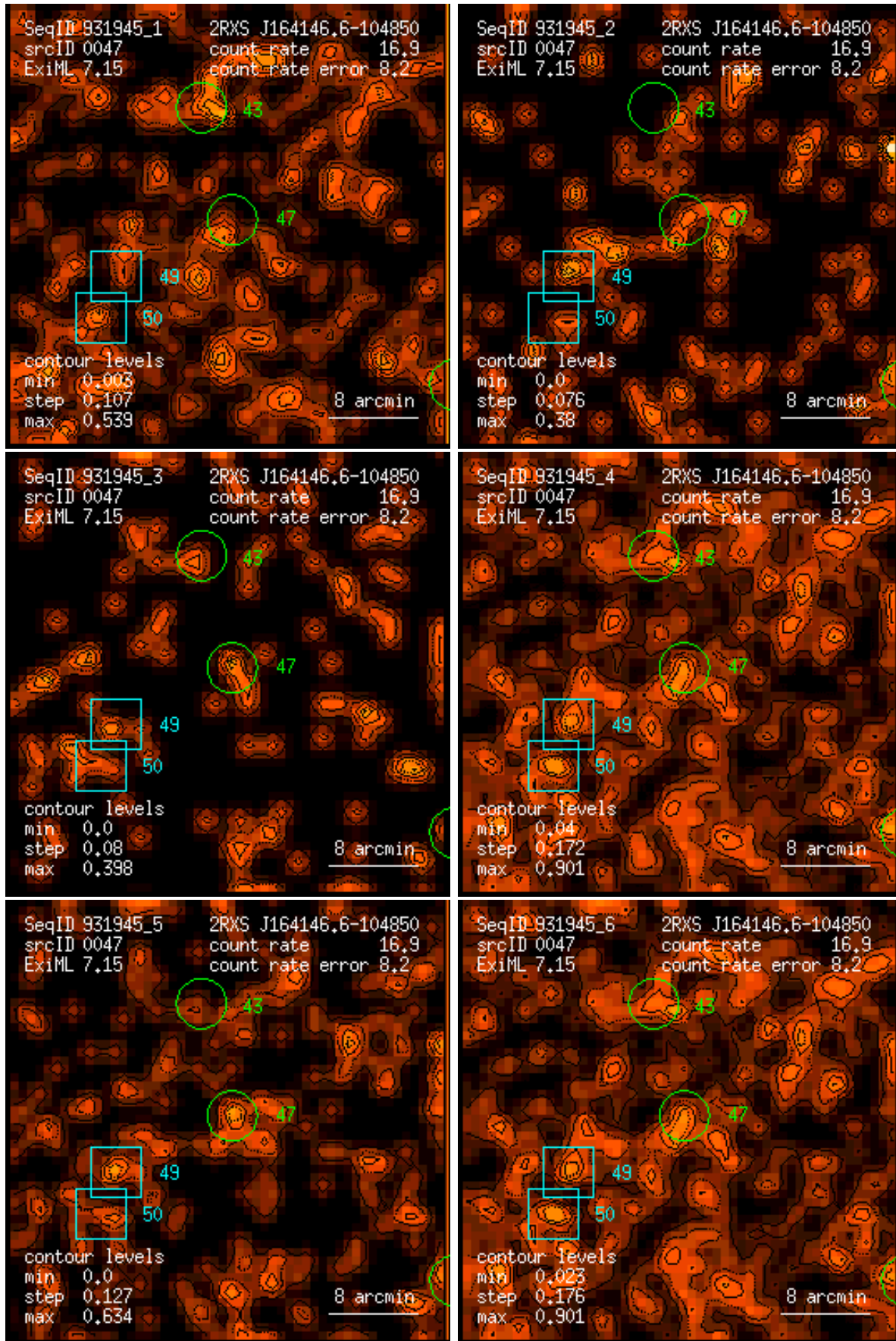
Figure 47: RASS 931945: detection 0047: band rate images, Gaussian filter: (1) PSPC channels 11 – 41, (2) 52 – 90, (3) 91 – 201, (4) 11 – 235, (5) 52 – 201, (6) 11 – 201. Broad band rates in counts/ks. Band rate contour levels in counts/ks/arcmin 2 .
