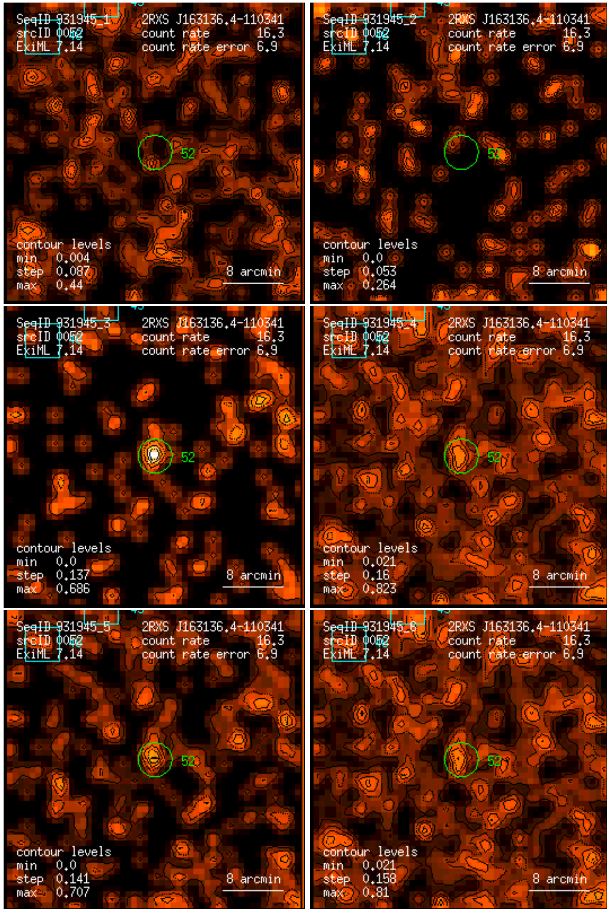
Figure 52: RASS 931945: detection 0052: band rate images, Gaussian filter: (1) PSPC channels 11 – 41, (2) 52 – 90, (3) 91 – 201, (4) 11 – 235, (5) 52 – 201, (6) 11 – 201. Broad band rates in counts/ks. Band rate contour levels in counts/ks/arcmin 2 .
