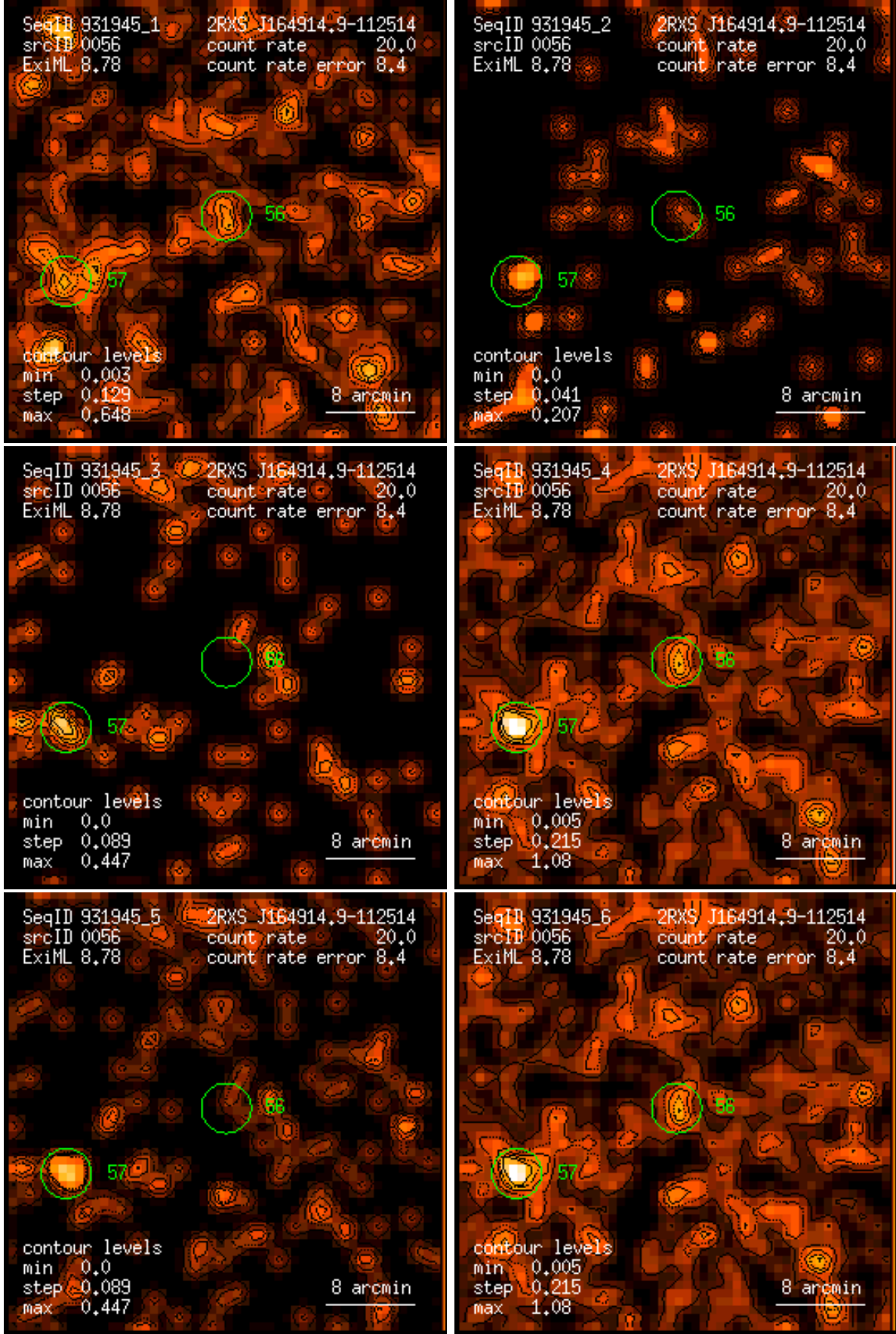
Figure 56: RASS 931945: detection 0056: band rate images, Gaussian filter: (1) PSPC channels 11 – 41, (2) 52 – 90, (3) 91 – 201, (4) 11 – 235, (5) 52 – 201, (6) 11 – 201. Broad band rates in counts/ks. Band rate contour levels in counts/ks/arcmin 2 .
