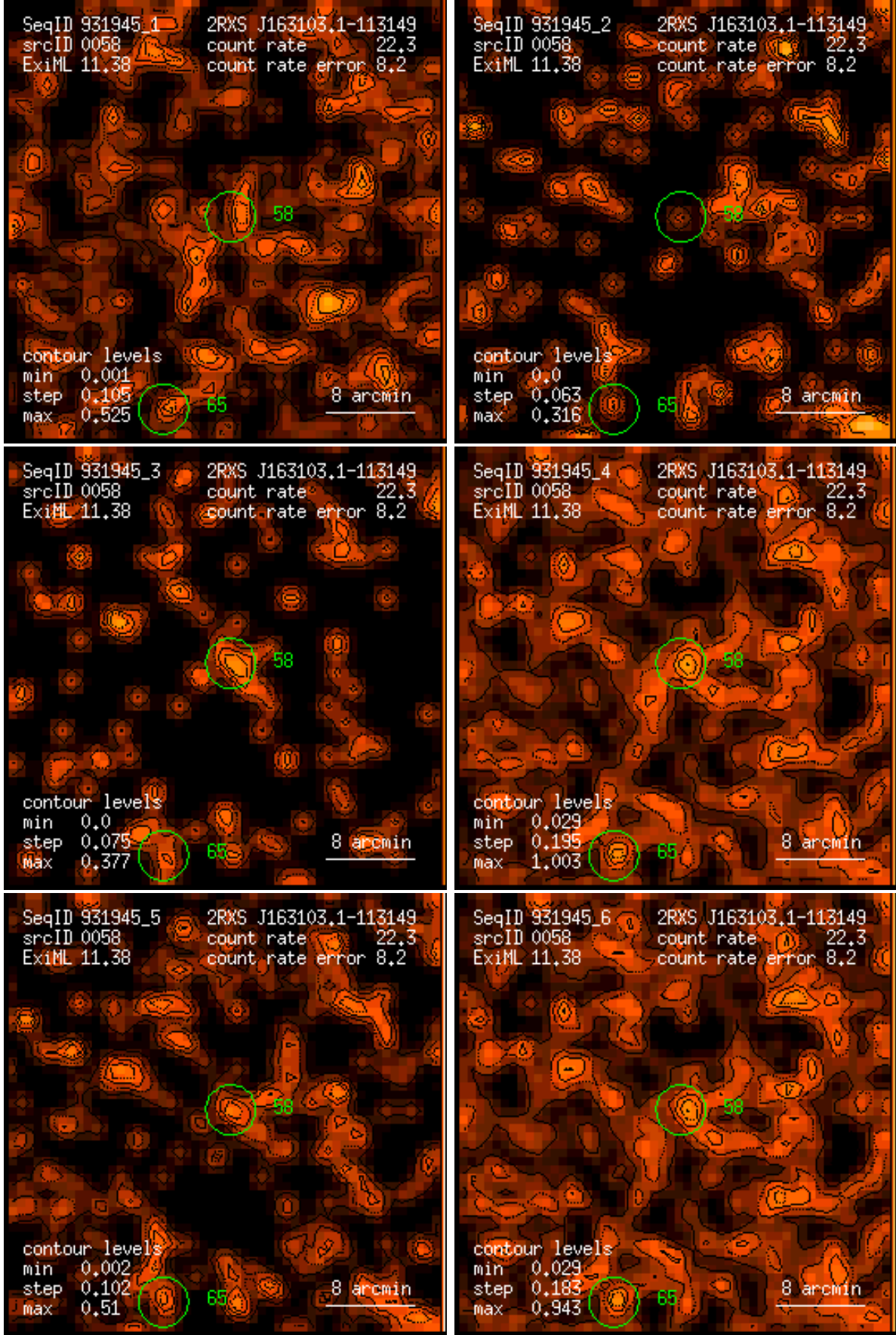
Figure 58: RASS 931945: detection 0058: band rate images, Gaussian filter: (1) PSPC channels 11 – 41, (2) 52 – 90, (3) 91 – 201, (4) 11 – 235, (5) 52 – 201, (6) 11 – 201. Broad band rates in counts/ks. Band rate contour levels in counts/ks/arcmin 2 .
