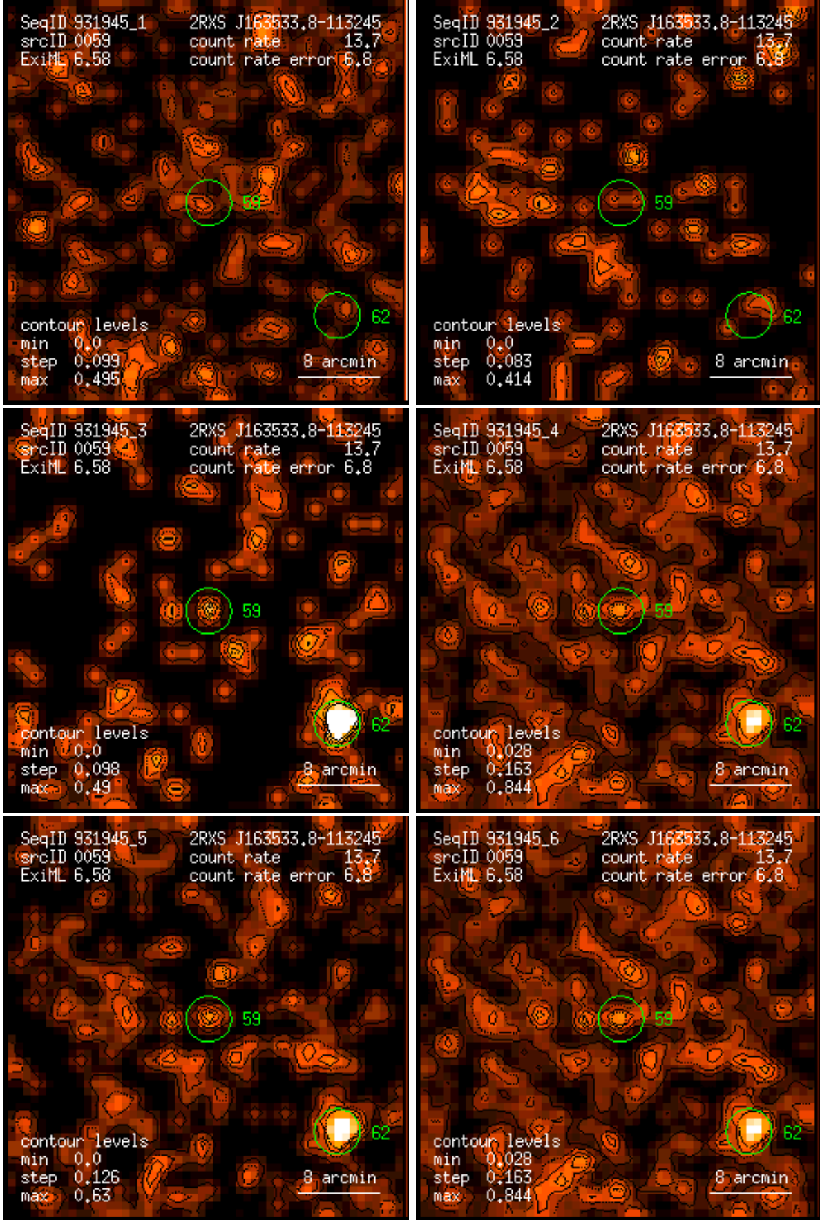
Figure 59: RASS 931945: detection 0059: band rate images, Gaussian filter: (1) PSPC channels 11 – 41, (2) 52 – 90, (3) 91 – 201, (4) 11 – 235, (5) 52 – 201, (6) 11 – 201. Broad band rates in counts/ks. Band rate contour levels in counts/ks/arcmin 2 .
