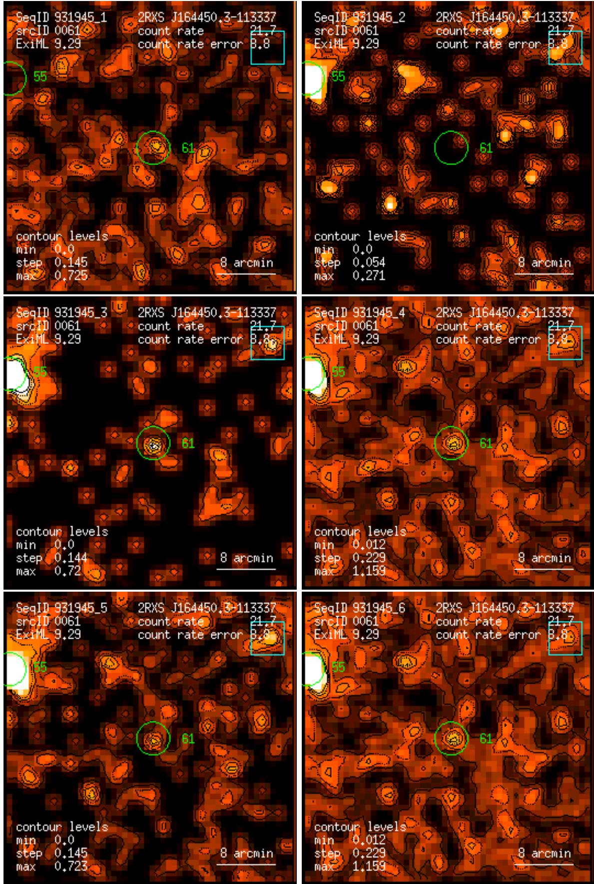
Figure 61: RASS 931945: detection 0061: band rate images, Gaussian filter: (1) PSPC channels 11 – 41, (2) 52 – 90, (3) 91 – 201, (4) 11 – 235, (5) 52 – 201, (6) 11 – 201. Broad band rates in counts/ks. Band rate contour levels in counts/ks/arcmin 2 .
