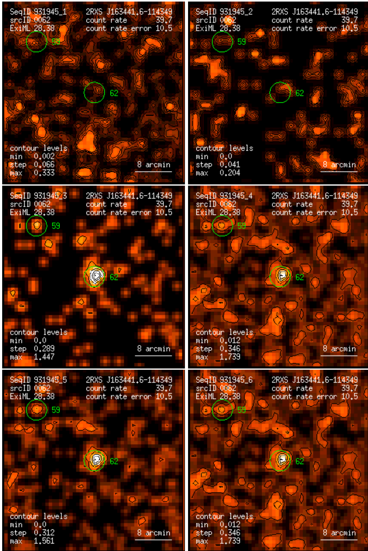
Figure 62: RASS 931945: detection 0062: band rate images, Gaussian filter: (1) PSPC channels 11 – 41, (2) 52 – 90, (3) 91 – 201, (4) 11 – 235, (5) 52 – 201, (6) 11 – 201. Broad band rates in counts/ks. Band rate contour levels in counts/ks/arcmin 2 .
