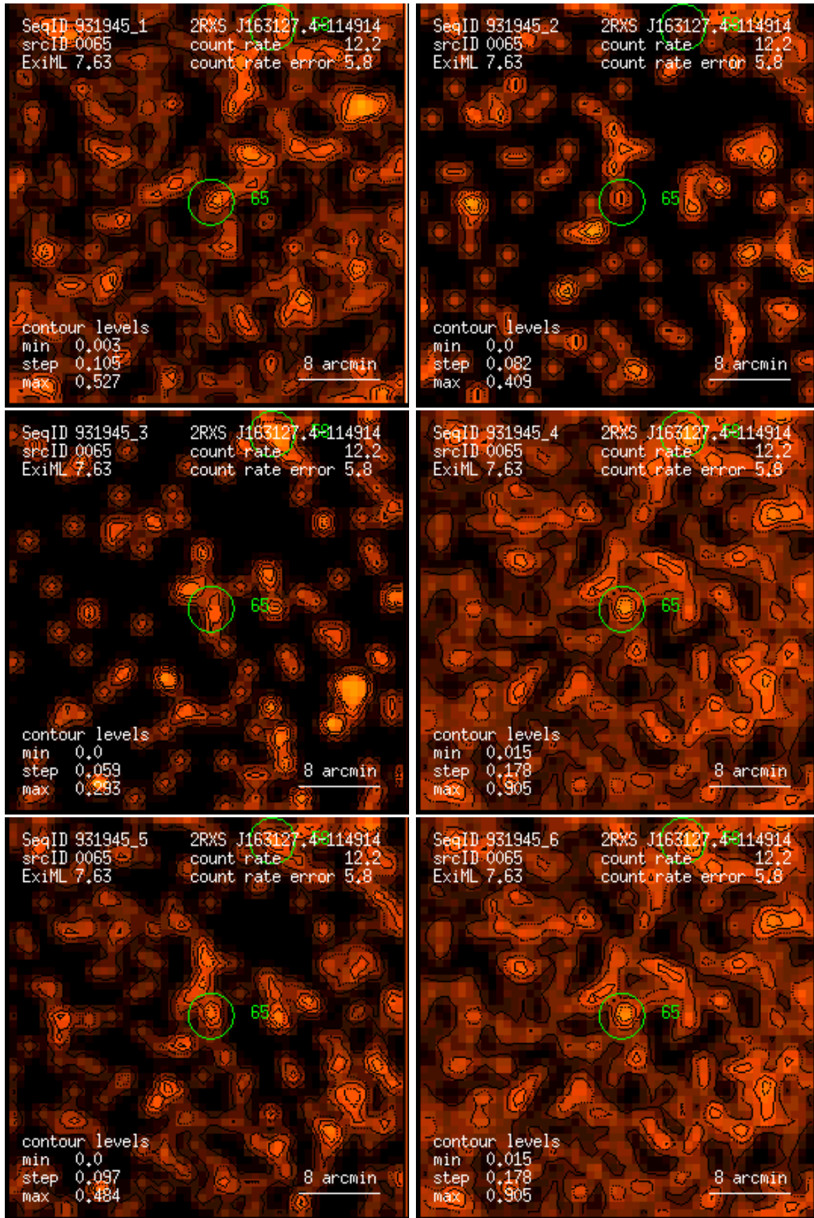
Figure 65: RASS 931945: detection 0065: band rate images, Gaussian filter: (1) PSPC channels 11 – 41, (2) 52 – 90, (3) 91 – 201, (4) 11 – 235, (5) 52 – 201, (6) 11 – 201. Broad band rates in counts/ks. Band rate contour levels in counts/ks/arcmin 2 .
