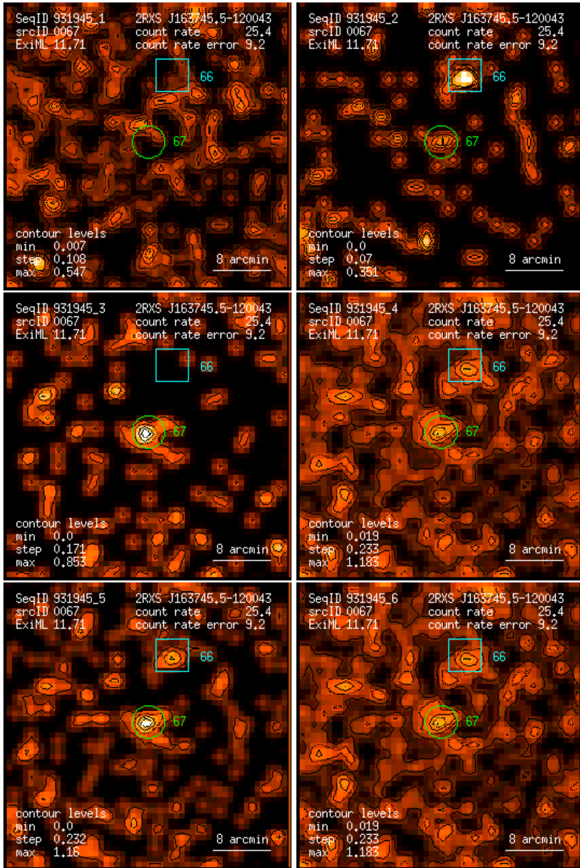
Figure 67: RASS 931945: detection 0067: band rate images, Gaussian filter: (1) PSPC channels 11 – 41, (2) 52 – 90, (3) 91 – 201, (4) 11 – 235, (5) 52 – 201, (6) 11 – 201. Broad band rates in counts/ks. Band rate contour levels in counts/ks/arcmin 2 .
