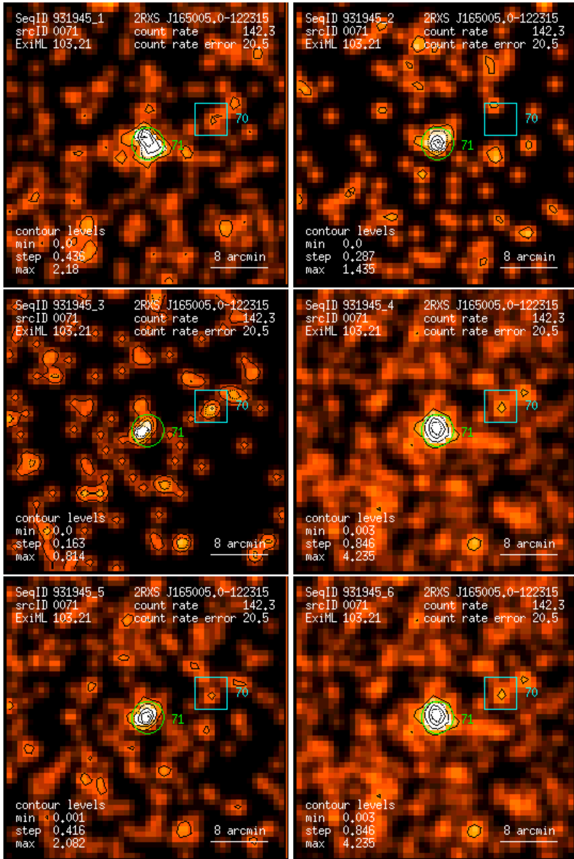
Figure 71: RASS 931945: detection 0071: band rate images, Gaussian filter: (1) PSPC channels 11 – 41, (2) 52 – 90, (3) 91 – 201, (4) 11 – 235, (5) 52 – 201, (6) 11 – 201. Broad band rates in counts/ks. Band rate contour levels in counts/ks/arcmin 2 .
