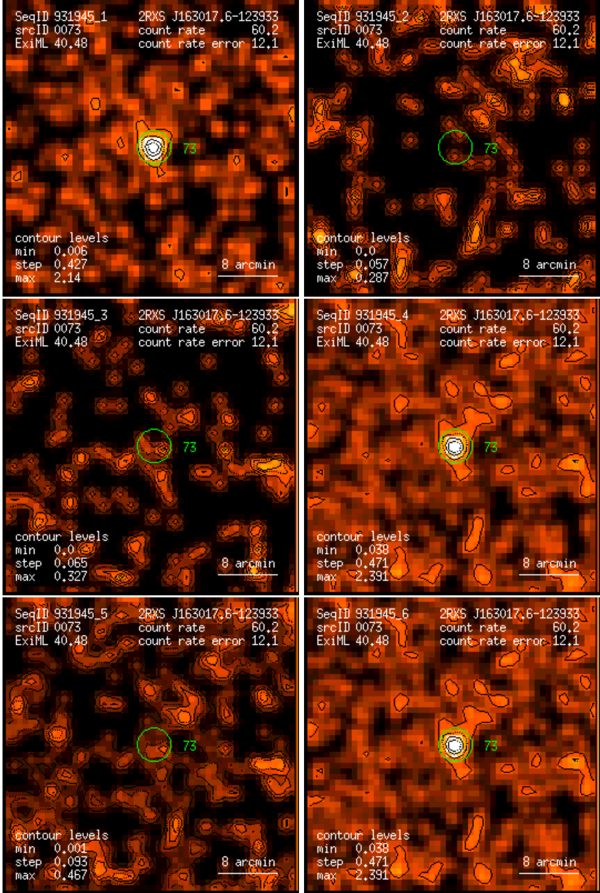
Figure 73: RASS 931945: detection 0073: band rate images, Gaussian filter: (1) PSPC channels 11 – 41, (2) 52 – 90, (3) 91 – 201, (4) 11 – 235, (5) 52 – 201, (6) 11 – 201. Broad band rates in counts/ks. Band rate contour levels in counts/ks/arcmin 2 .
