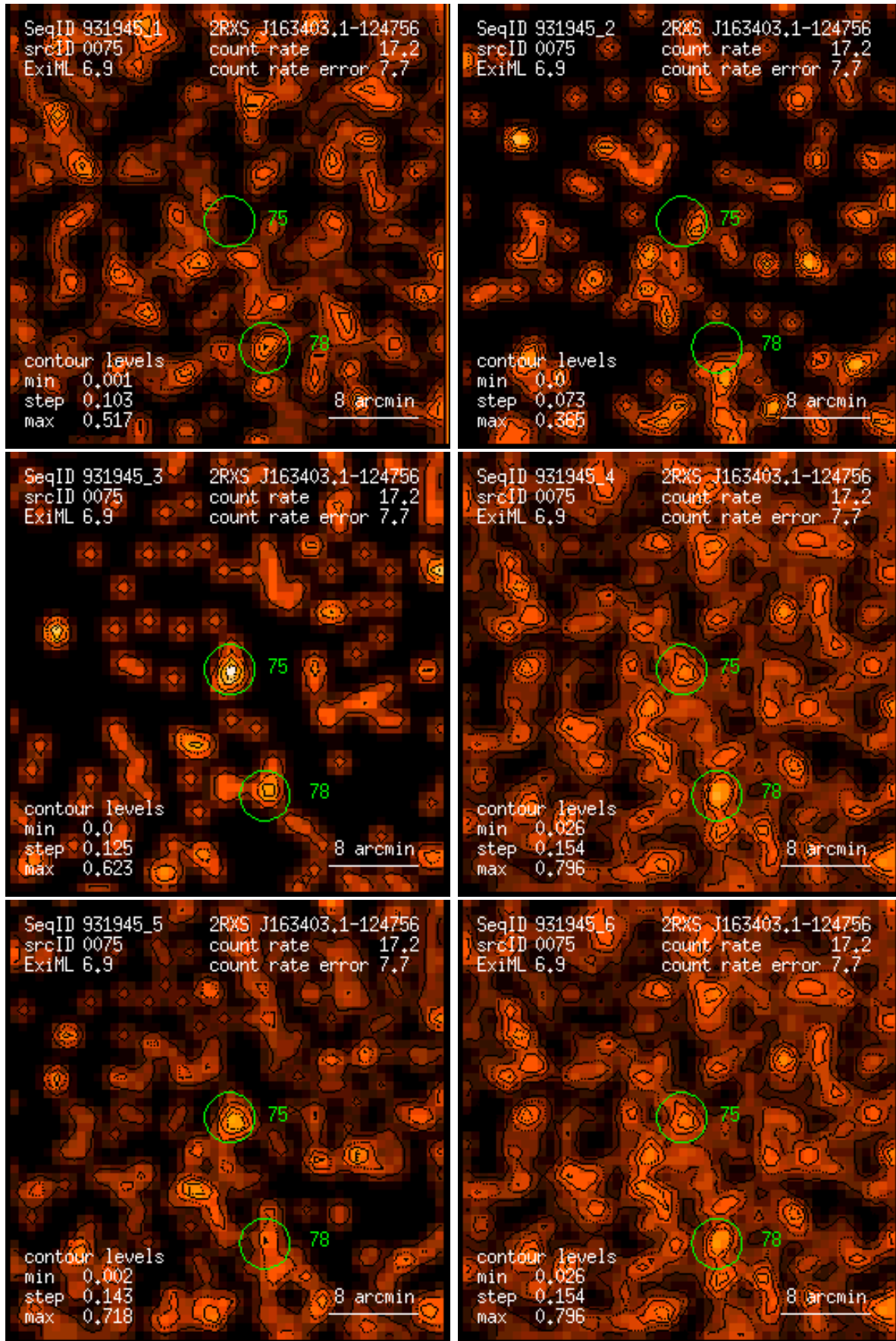
Figure 75: RASS 931945: detection 0075: band rate images, Gaussian filter: (1) PSPC channels 11 – 41, (2) 52 – 90, (3) 91 – 201, (4) 11 – 235, (5) 52 – 201, (6) 11 – 201. Broad band rates in counts/ks. Band rate contour levels in counts/ks/arcmin 2 .
