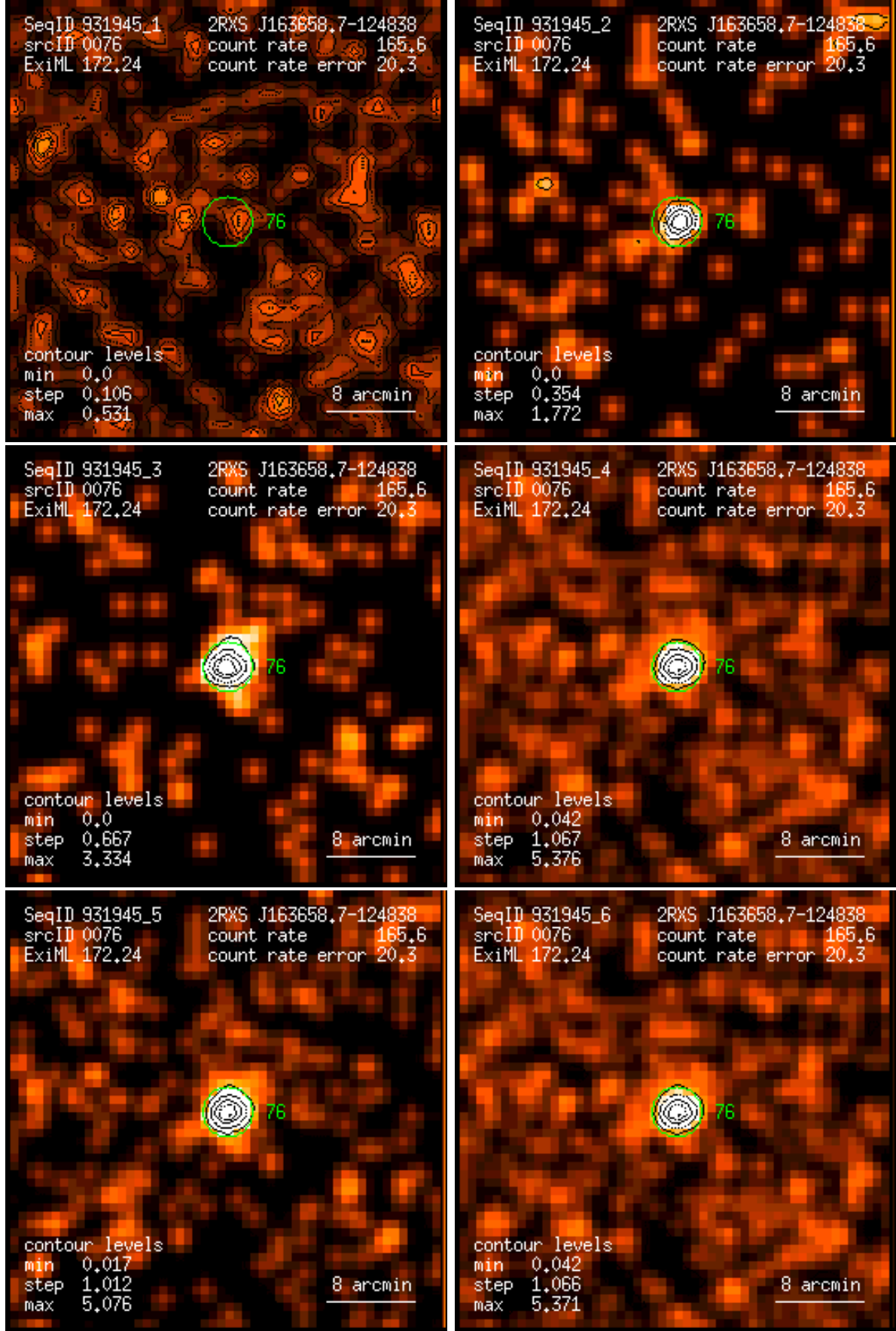
Figure 76: RASS 931945: detection 0076: band rate images, Gaussian filter: (1) PSPC channels 11 – 41, (2) 52 – 90, (3) 91 – 201, (4) 11 – 235, (5) 52 – 201, (6) 11 – 201. Broad band rates in counts/ks. Band rate contour levels in counts/ks/arcmin 2 .
